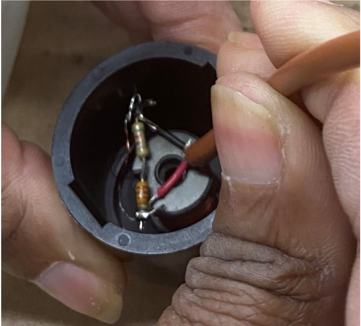
Figure 1 Internal photo of HRE inductive loop antenna.
