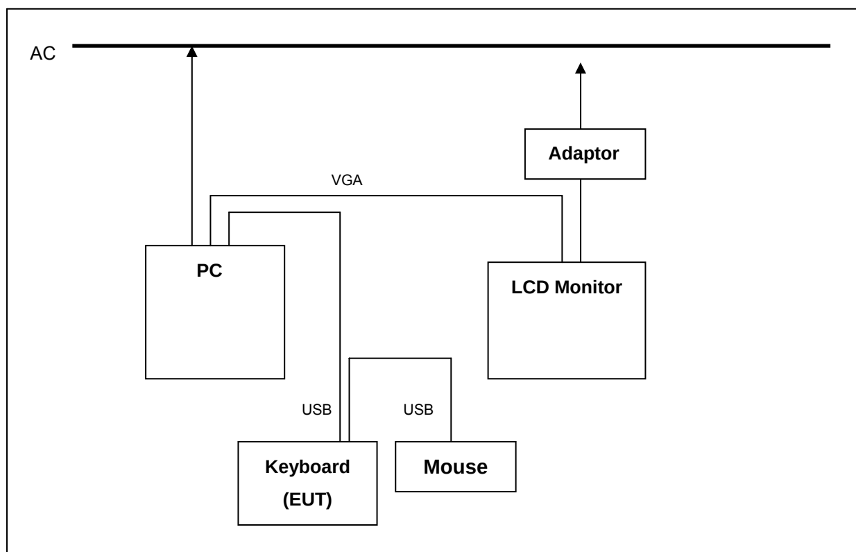
[ System Block Diagram of Test Configuration ]
