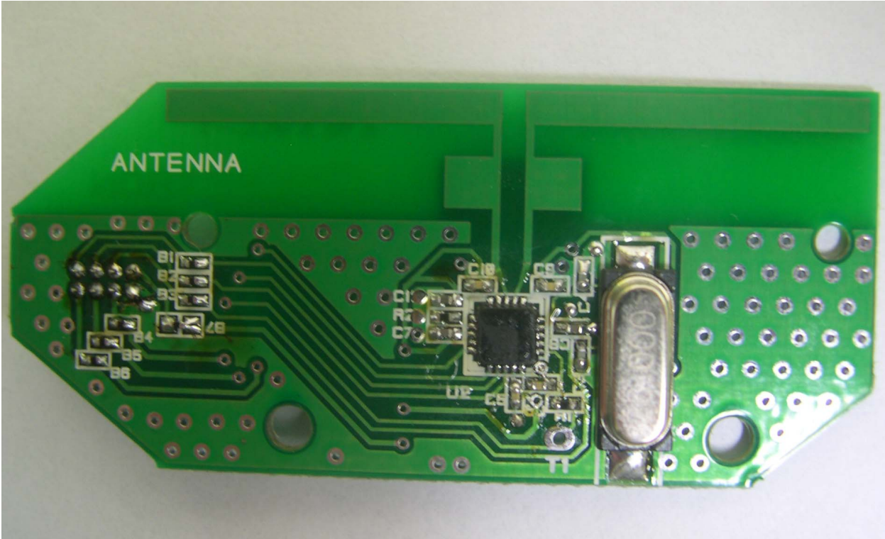
<Photograph 4: Front View – RF board>
