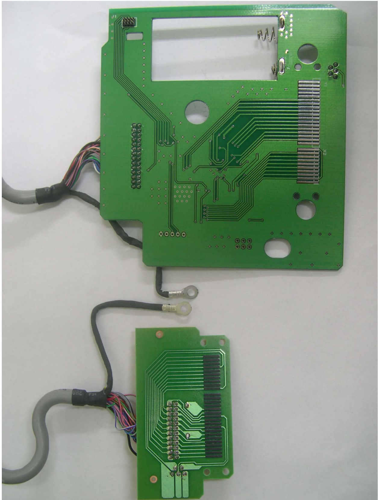
<Photograph 3: Rear View – Main board>
