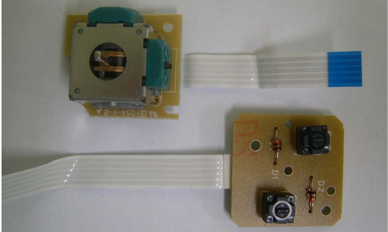
<Photograph 6: Front View – SUB-board: Track ball, function key>
