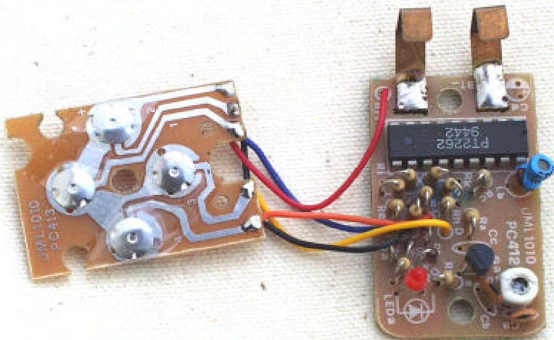
FCC ID: GJM1010 FRONT VIEW OF THE PRINTED WIRING BOARD
