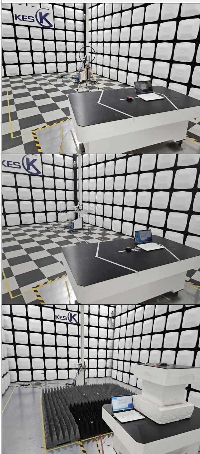
Radiated test
