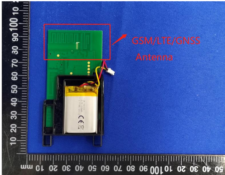
Battery TOP VIEW
