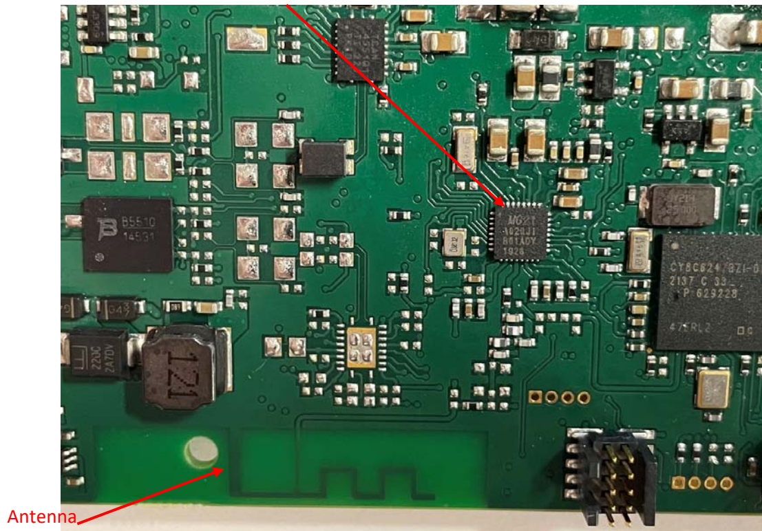
Bluetooth LE Chip with Antenna View
