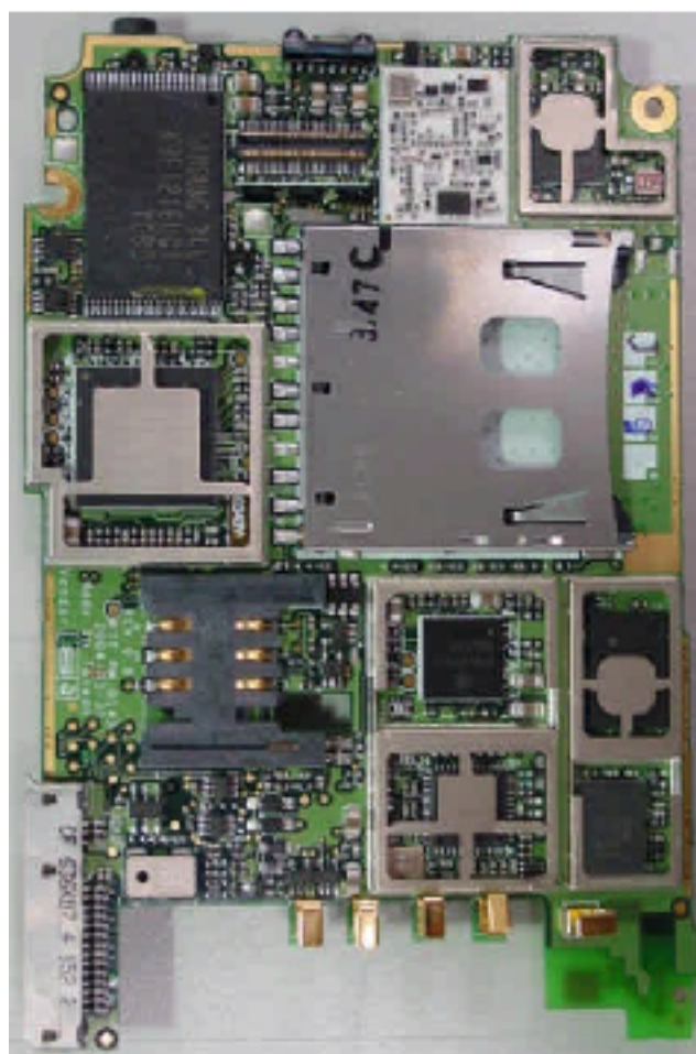
Front View Covers Removed
