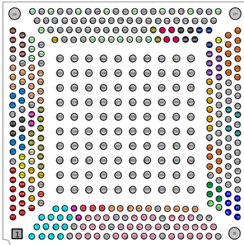
Figure 3-1 Antenna port location
