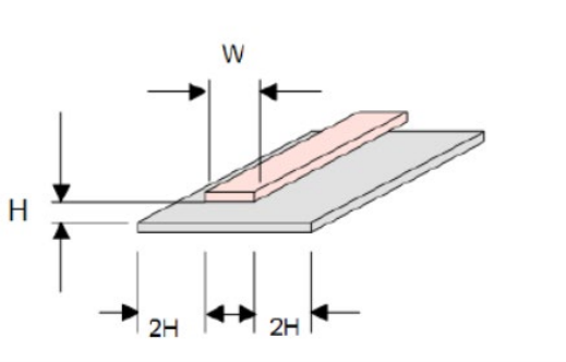
Figure 3-3 Complete structure of the microstrip
