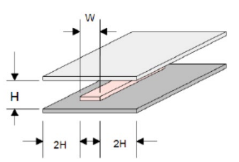
Figure 3-4 Complete structure of the stripline
