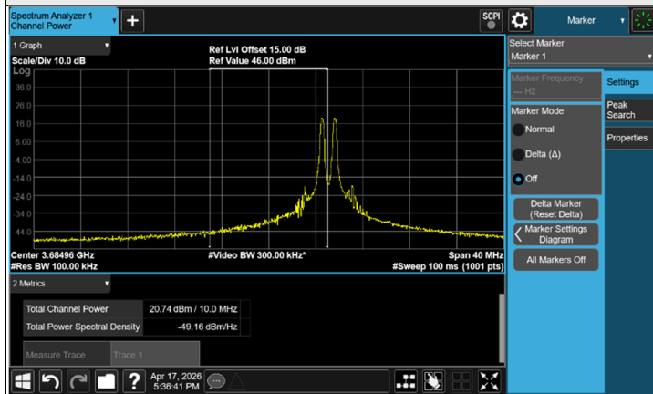
QPSK CH 56591 (3685.1 MHz)
