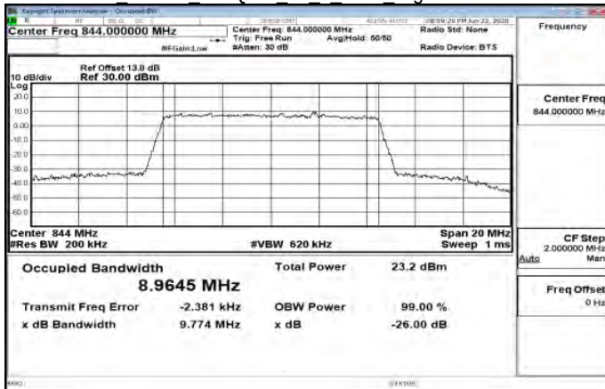
Band5 10MHz 256QAM 50 0 Main HighCH20600-844
