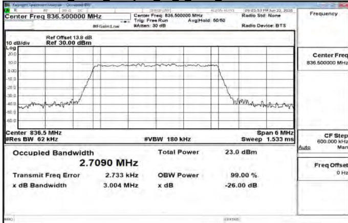
Band5 3MHz 256QAM 15 0 Main MidCH20525-836.5
