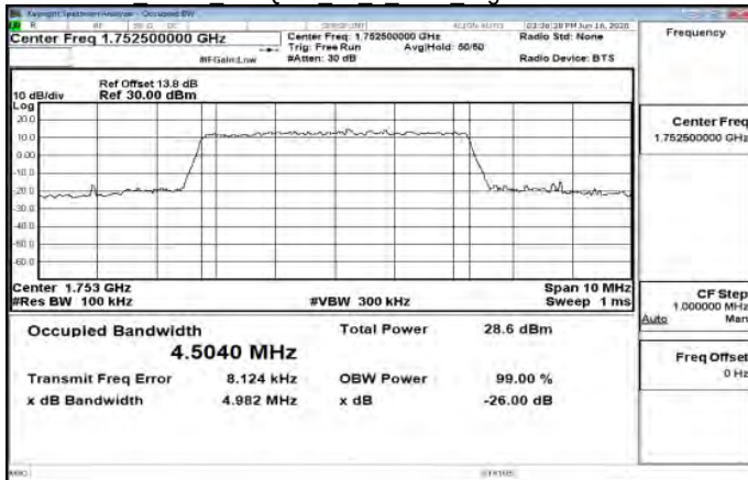
Band4 5MHz 256QAM 25 0 Main HighCH20375-1752.5
