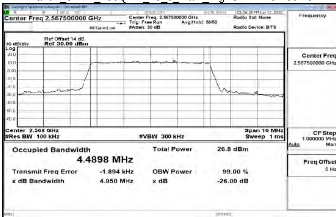
Band7 5MHz 256QAM 25 0 Main HighCH21425-2567.5
