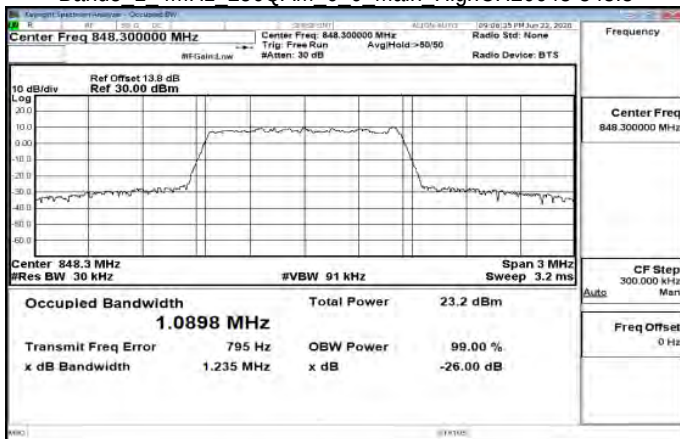
Band5 1 4MHz 256QAM 6 0 Main HighCH20643-848.3
