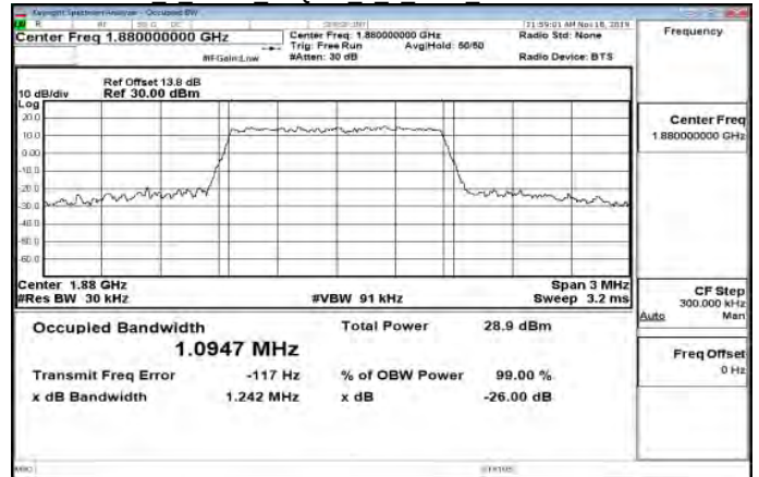
Band2 1 4MHz 64QAM 6 0 Main MidCH18900-1880
