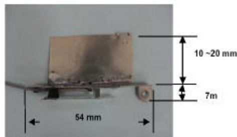
AUX antenna dimensioned drawing
