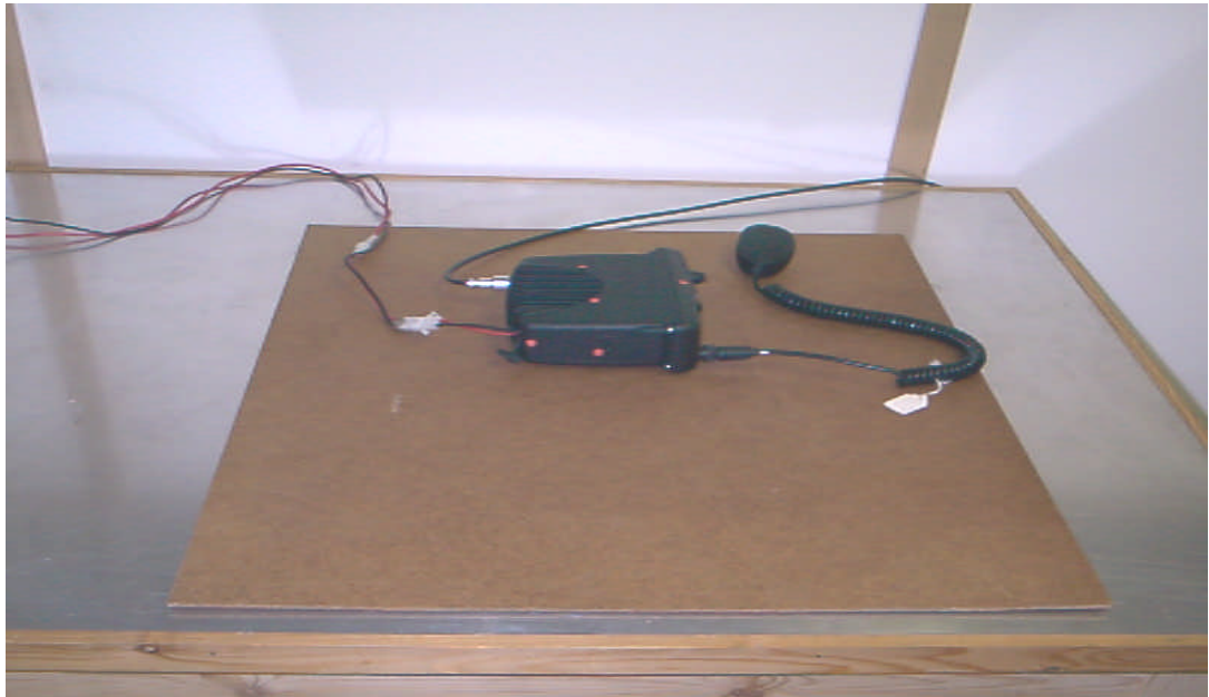
PHOTOGRAPH 8 Close up side view of RD62 showing ESD test points
