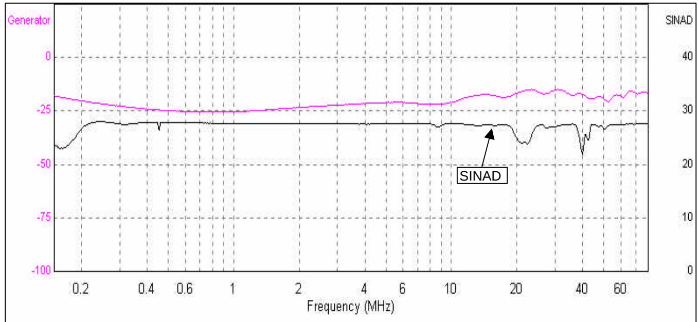
PLOT 11 Conducted Immunity measurement scan on the +ve supply line of the RD62 in receive mode of operation
