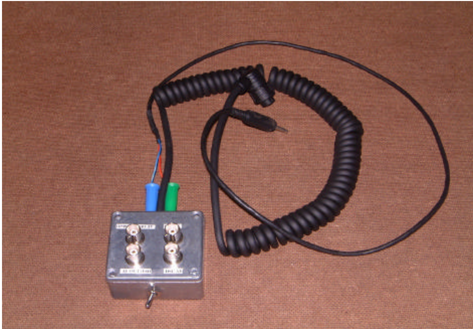
PHOTOGRAPH 7 General view of ptt connection box used during testing
