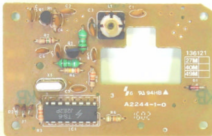
Model No. 136121A The top view of tx's PCB
