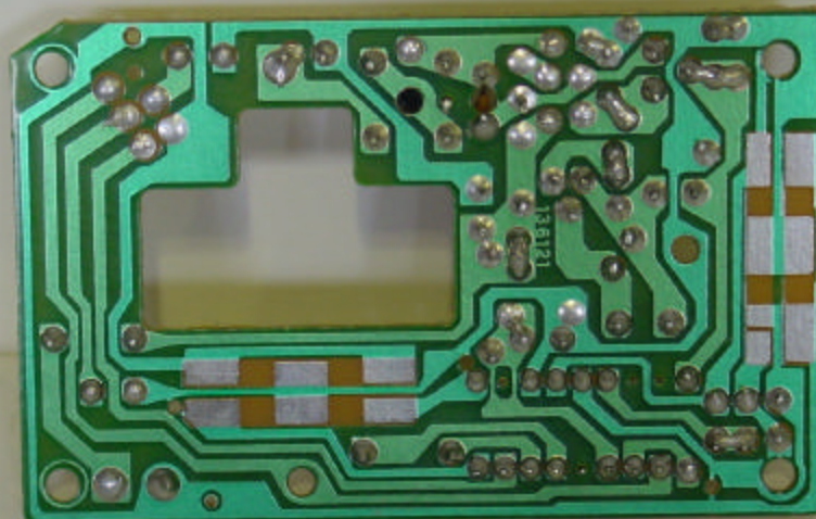
Model No. 136121A The bottom view of tx's PCB
