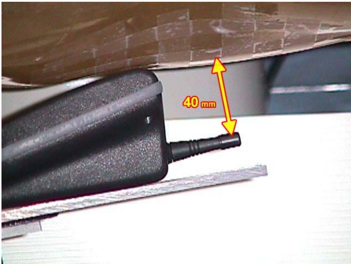
< Close-up view – Waist with the EUT parallel to the phantom and the display faced inward to the phantom >
