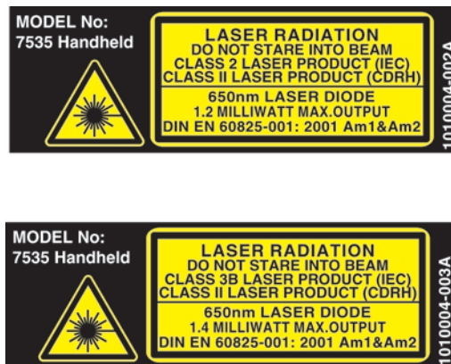
Figure 1.5 Laser Warning Labels
