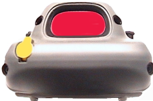
Figure 1.4 Scanner Window
