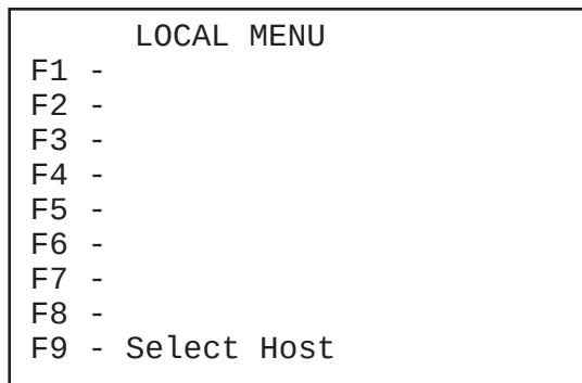
Figure 6.3 Local Menu
