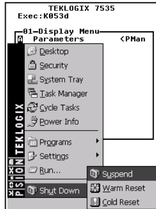
Figure 4.12 Shutdown Sub-Menu
