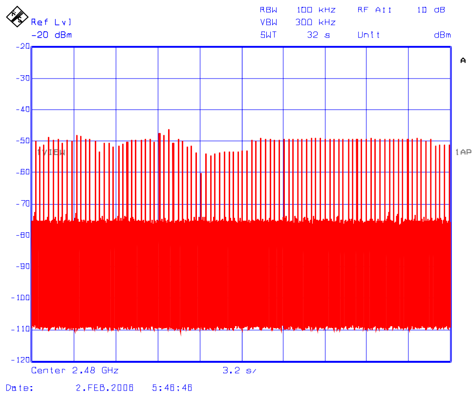
Plot 5.9.4.7: Time of Occupancy Test Frequency: 2480 MHz
