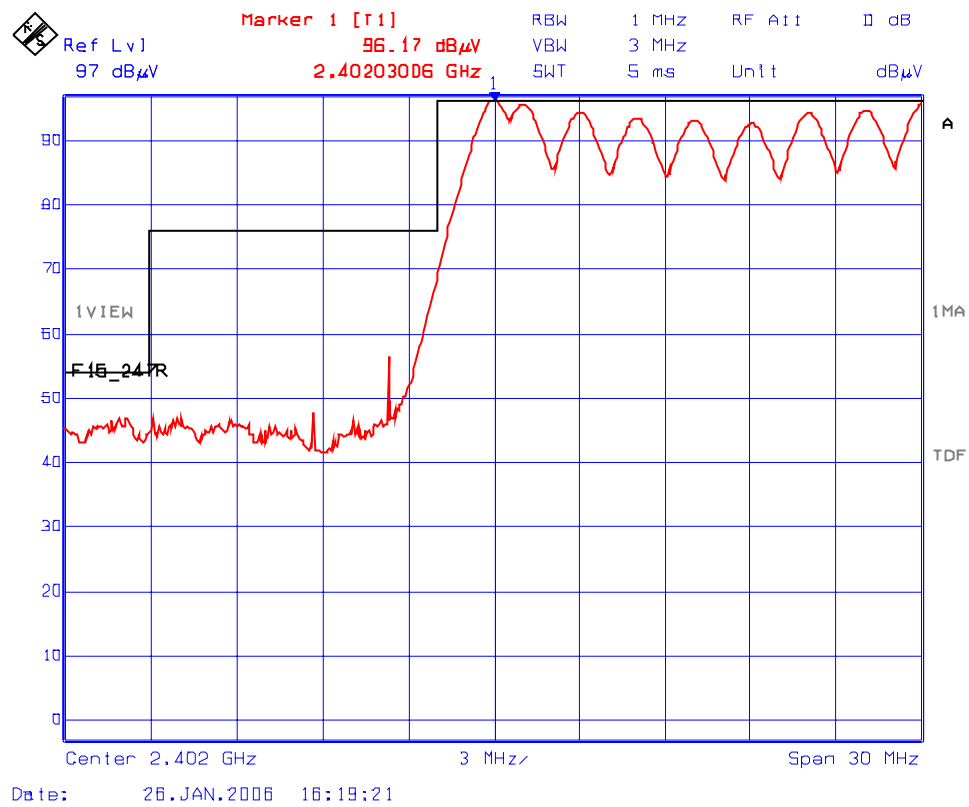
Plot 5.7.5.1.3 Band-Edge Radiated Emissions @ 3 meters, Vertical Polarization Low End of Frequency Band - Frequency Hopping Enabled
