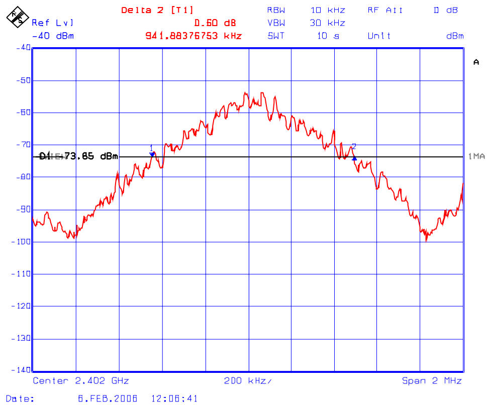
Plot 5.5.5.1.1: 20 dB Bandwidth Test Frequency: 2402 MHz
