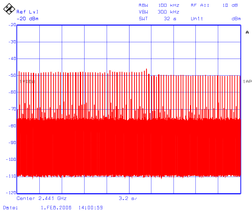
Plot 5.9.4.5: Time of Occupancy Test Frequency: 2441 MHz
