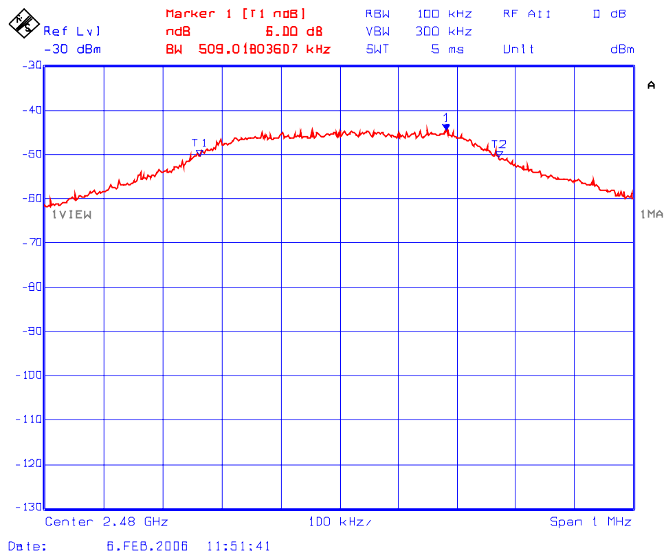
Plot 5.5.5.2.3: 6 dB Bandwidth Test Frequency: 2480 MHz
