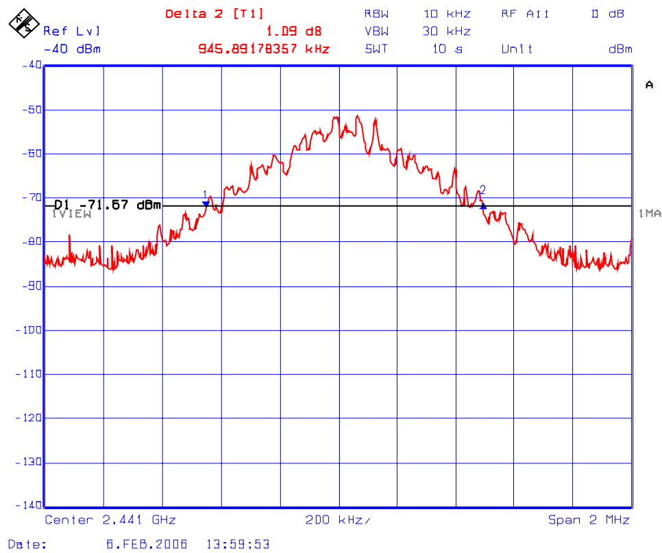
Plot 5.5.5.1.2: 20 dB Bandwidth Test Frequency: 2441 MHz
