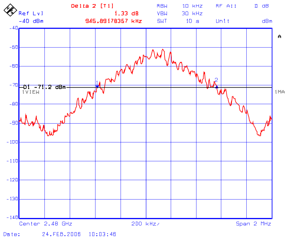
Plot 5.5.5.1.3: 20 dB Bandwidth Test Frequency: 2480 MHz
