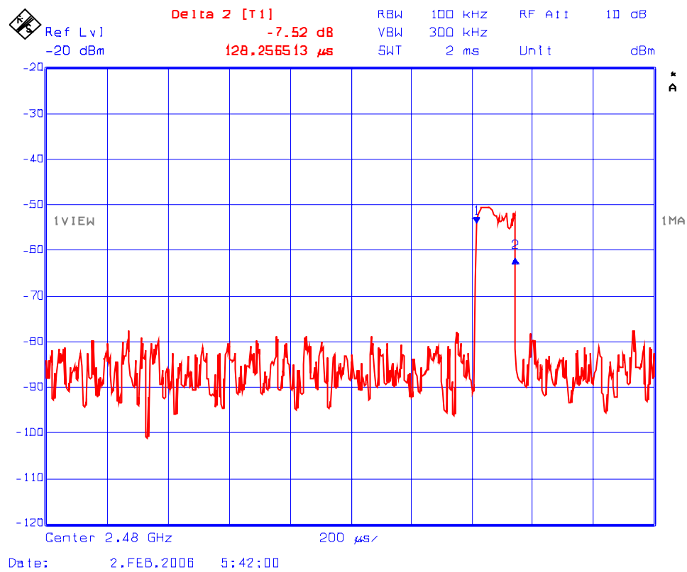
Plot 5.9.4.6: Time of Occupancy Test Frequency: 2480 MHz
