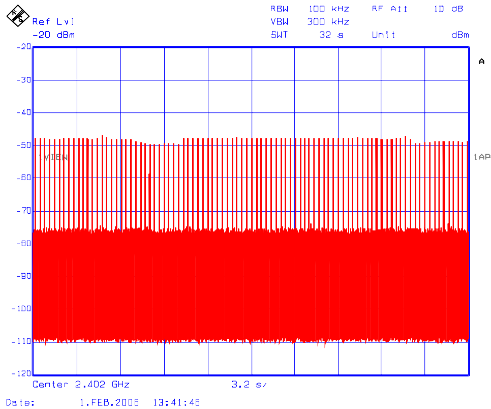
Plot 5.9.4.3: Time of Occupancy Test Frequency: 2402 MHz
