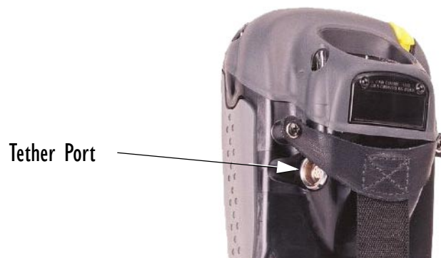
Figure 1.4 The Tether Port
