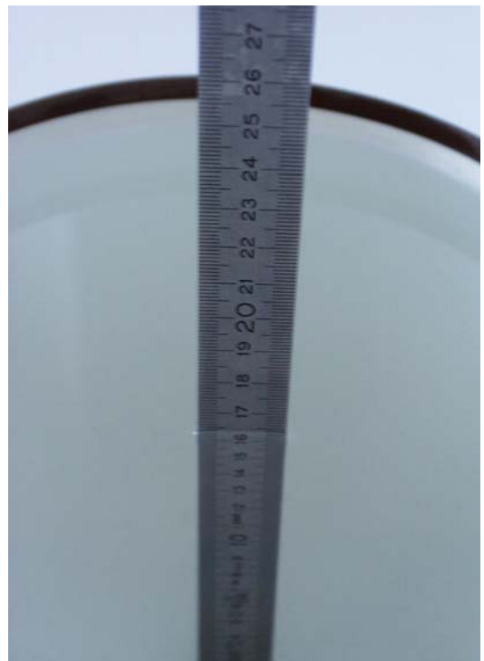
Fig. 48: Liquid depth for PCS 1900 and WCDMA II Head measurements
