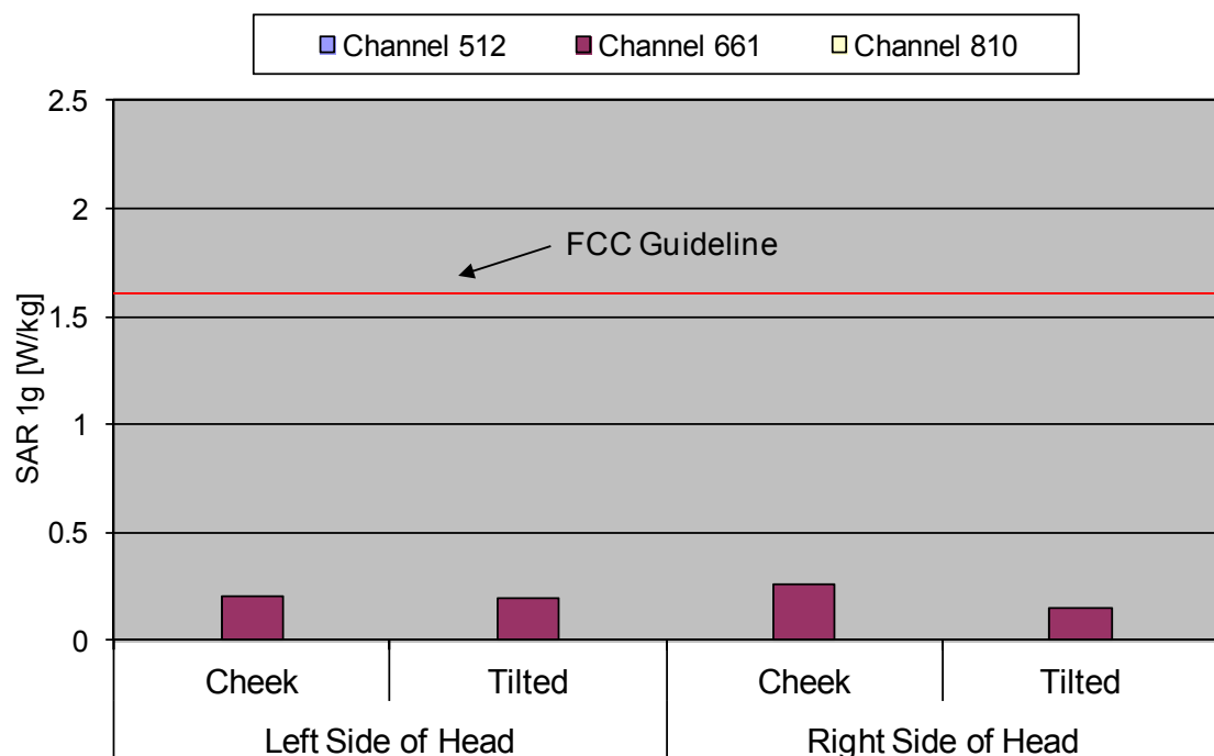
Fig. 9: The measured head SAR values for the PSION 7545MBW for PCS 1900 in head configuration, in comparison to the FCC exposure limit.
