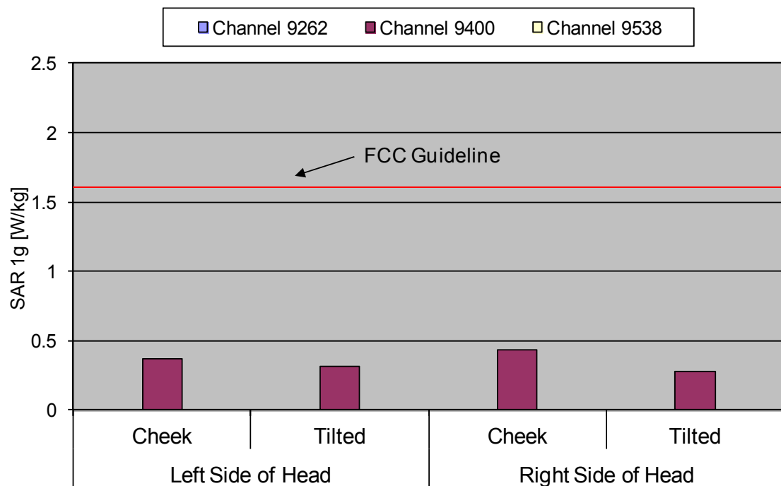
Fig. 11: The measured head SAR values for the PSION 7545MBW for WCDMA II (FDD) in head configuration, in comparison to the FCC exposure limit.
