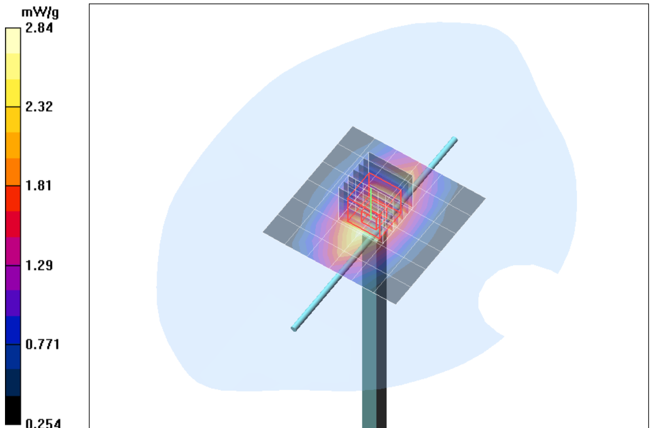
Fig. 20: Validation measurement 835 MHz (GSM 850) Head (December 22, 2011), coarse grid. Ambient Temperature: 21.6^\circ \text{ C} , Liquid Temperature: 21.3^\circ \text{ C} .
