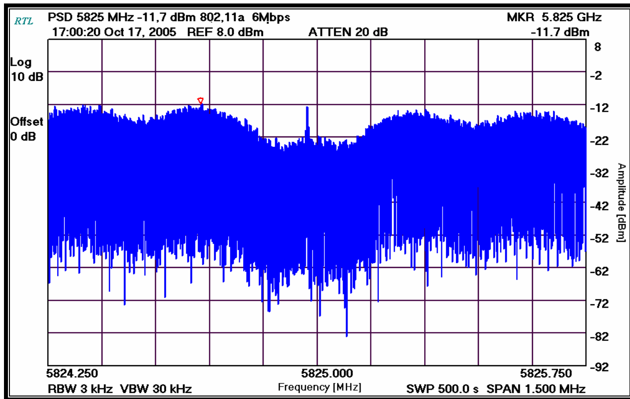
Plot 22-3: Power Spectral Density: Channel 165 (5825 MHz – 6 Mbps)
