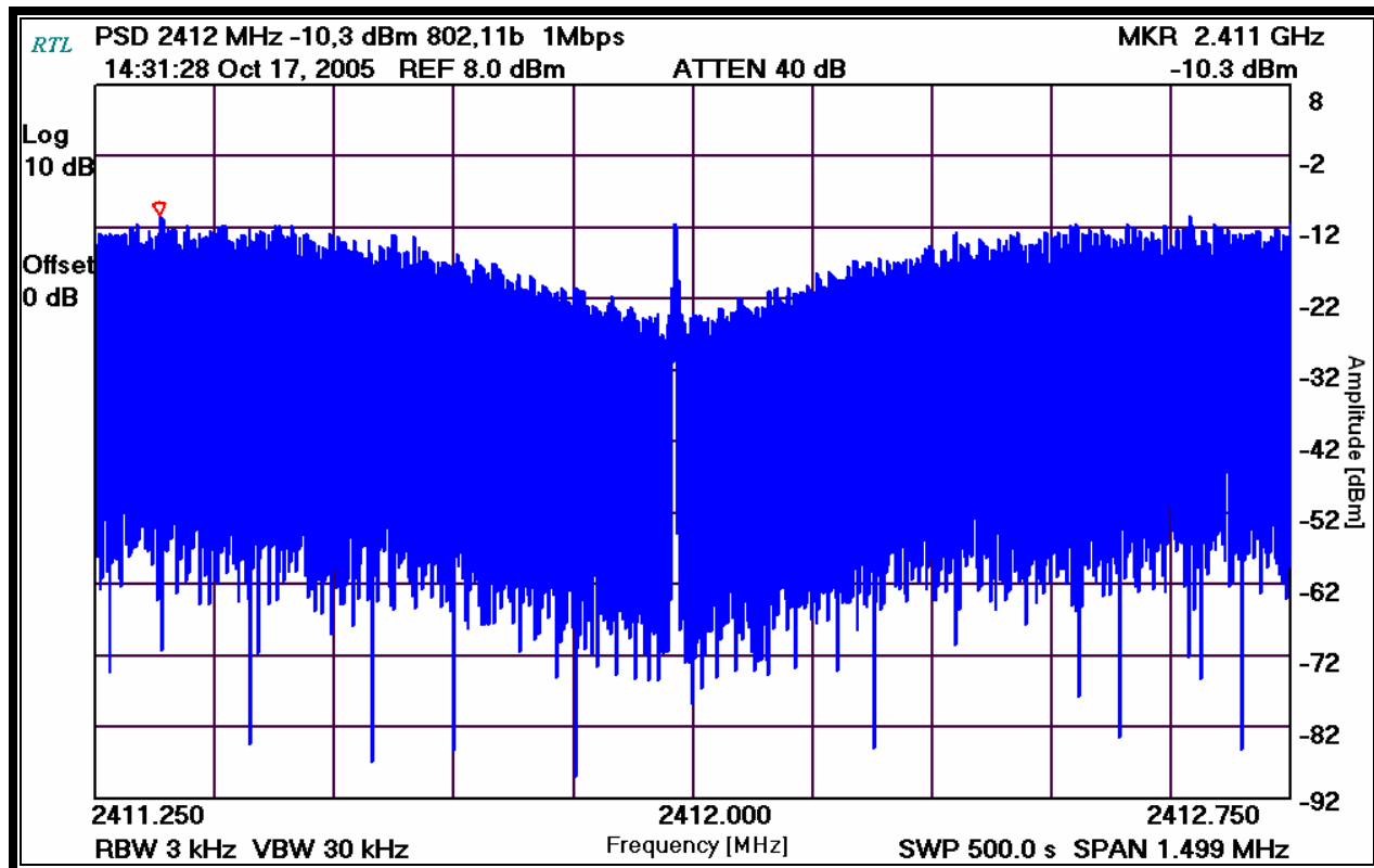
Plot 7-8: Power Spectral Density: Channel 1 (2412 MHz – 1 Mbps)
