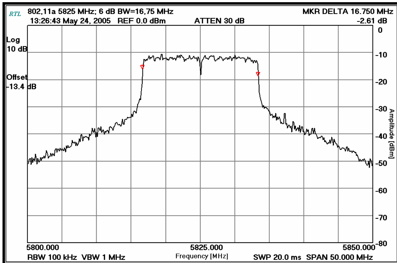
Plot 20-3: 6 dB Bandwidth (TX Frequency: 5825 MHz – 6 Mbs)
