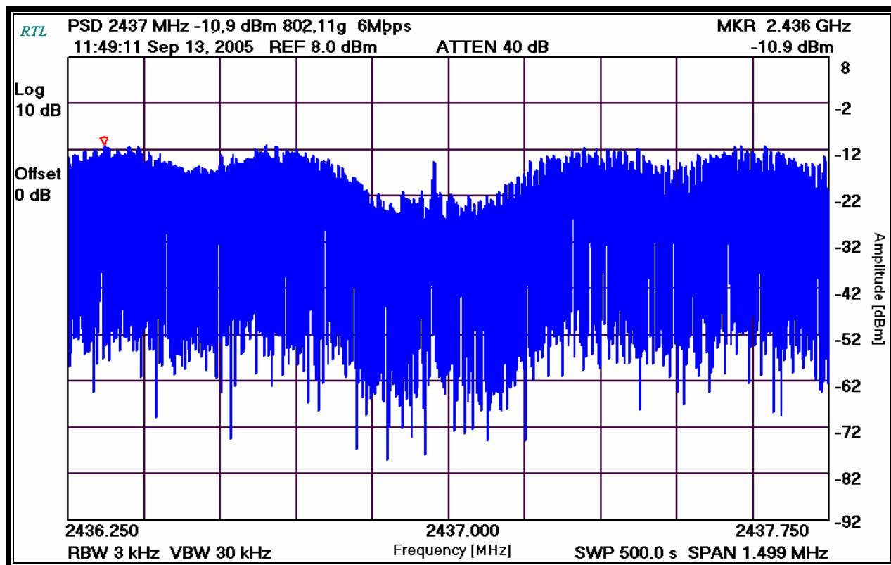
Plot 7-5: Power Spectral Density: Channel 6 (2437 MHz – 6 Mbps)
