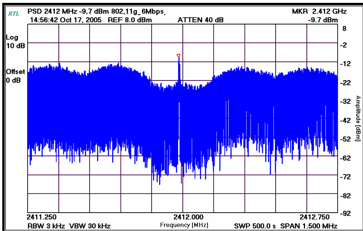
Plot 7-11: Power Spectral Density: Channel 1 (2412 MHz – 6 Mbps)
