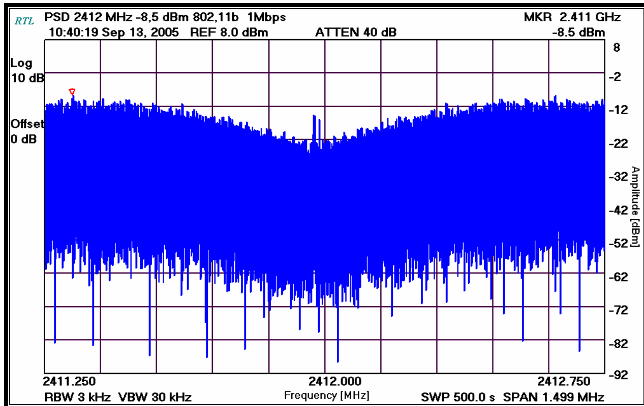
Plot 7-1: Power Spectral Density: Channel 1 (2412 MHz – 1 Mbps)
