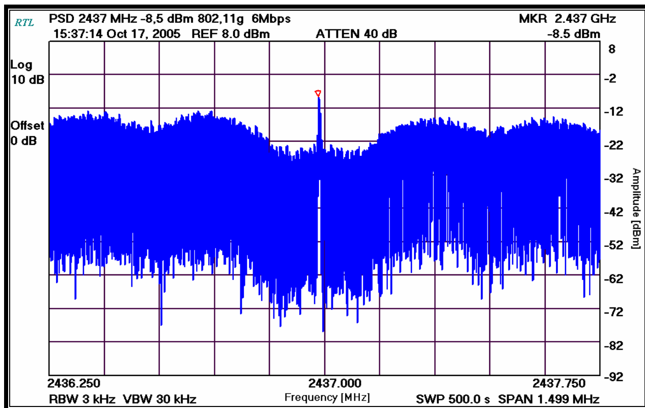
Plot 7-12: Power Spectral Density: Channel 6 (2437 MHz – 6 Mbps)
