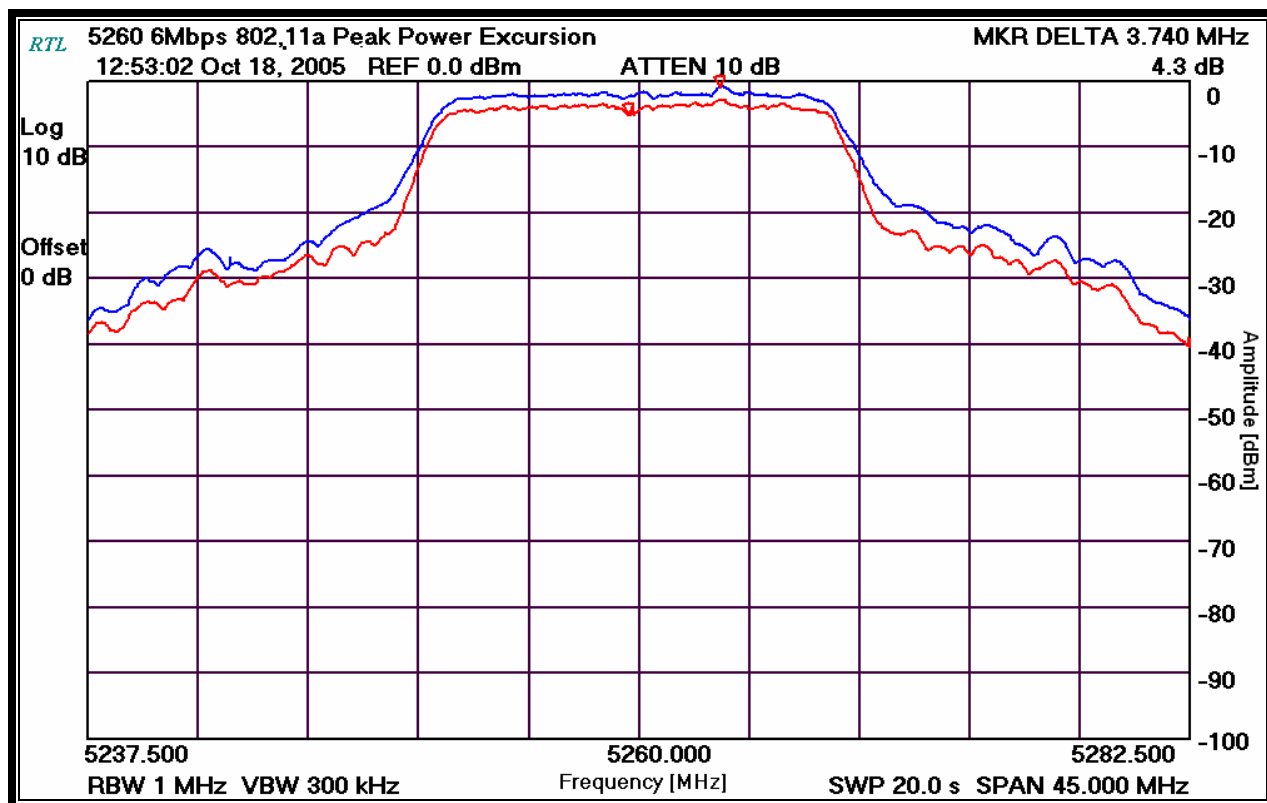
Plot 15-4: Peak Power Excursion: Channel 52 (5260 MHz – 6 Mb/s)
