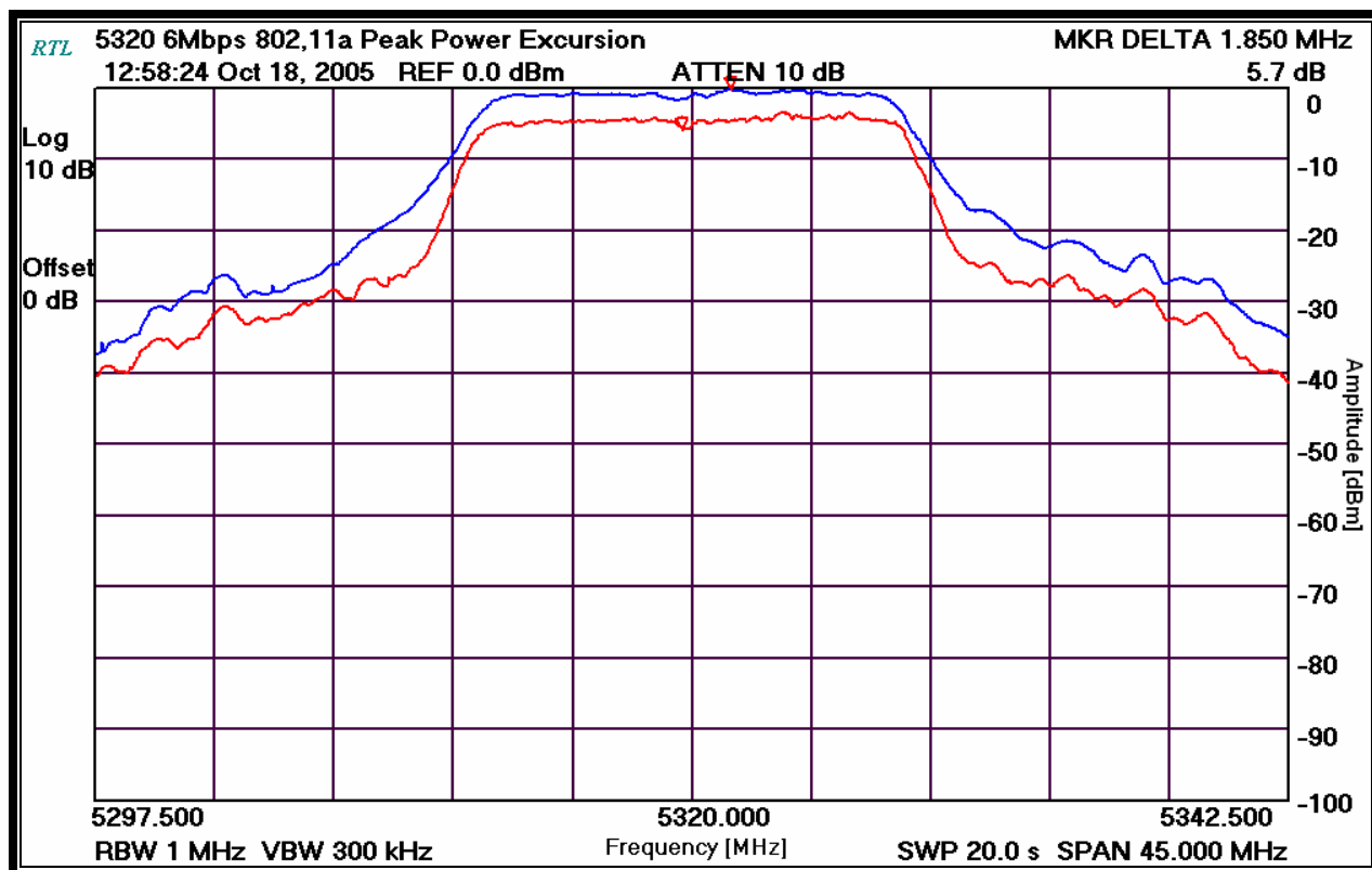
Plot 15-6: Peak Power Excursion: Channel 64 (5320 MHz – 6 Mb/s)
