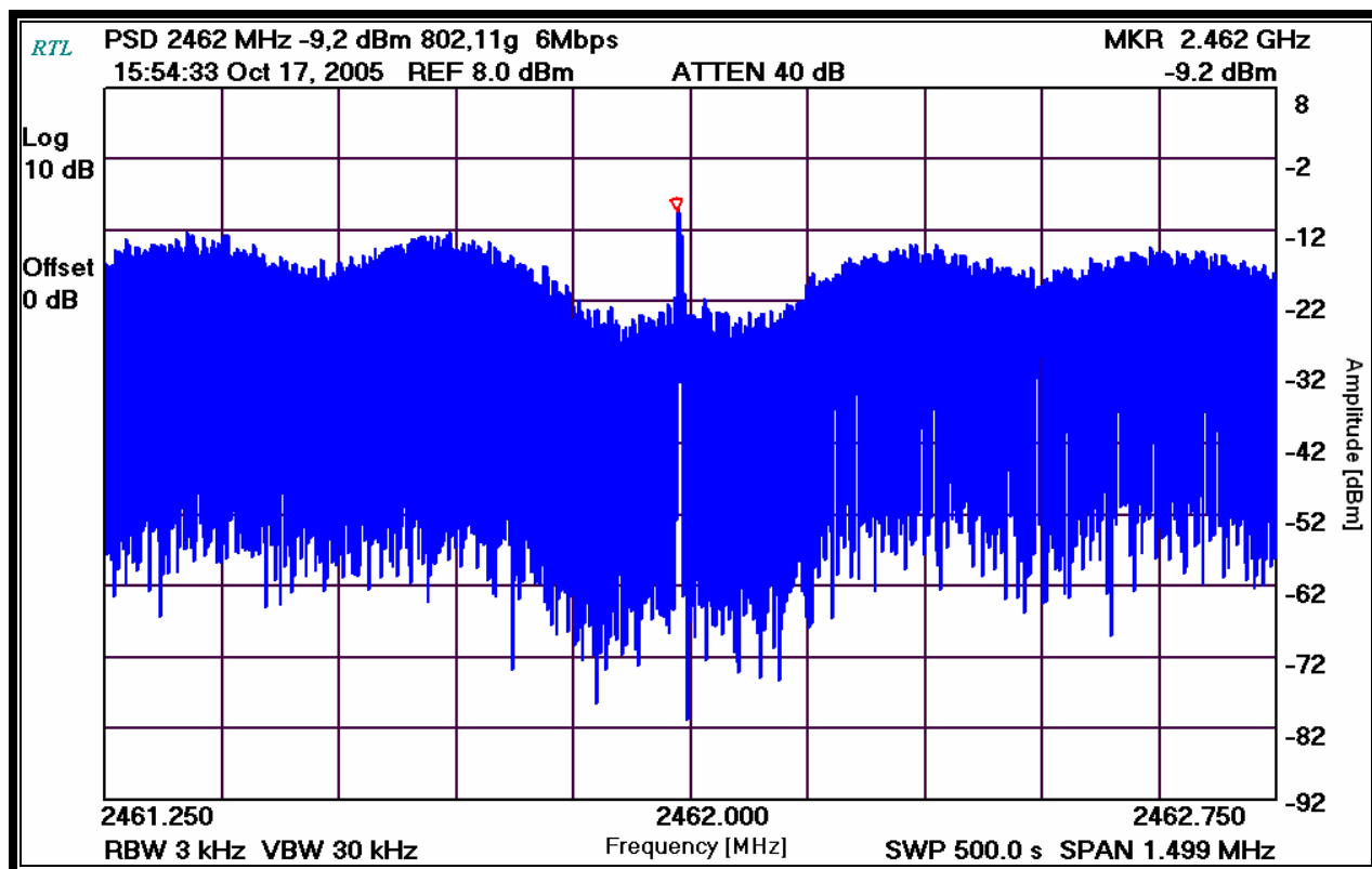
Plot 7-14: Power Spectral Density: Channel 11 (2462 MHz – 6 Mbps)
