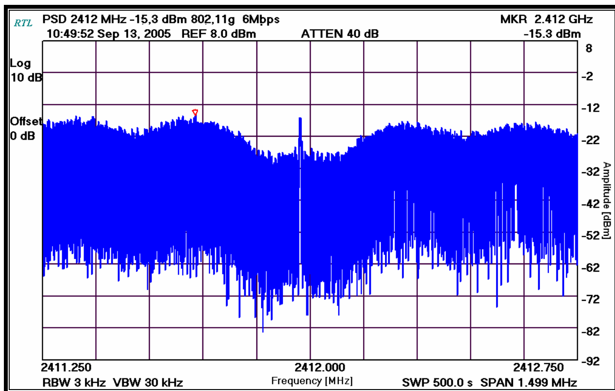
Plot 7-4: Power Spectral Density: Channel 1 (2412 MHz – 6 Mbps)
