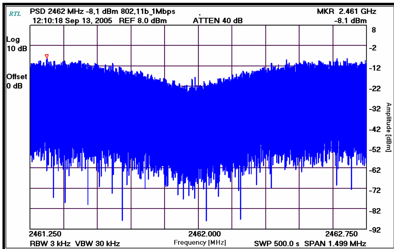
Plot 7-3: Power Spectral Density: Channel 11 (2462 MHz – 1 Mbps)
