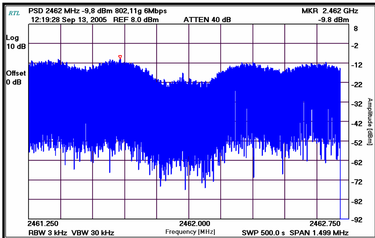
Plot 7-7: Power Spectral Density: Channel 11 (2462 MHz – 6 Mbps)
