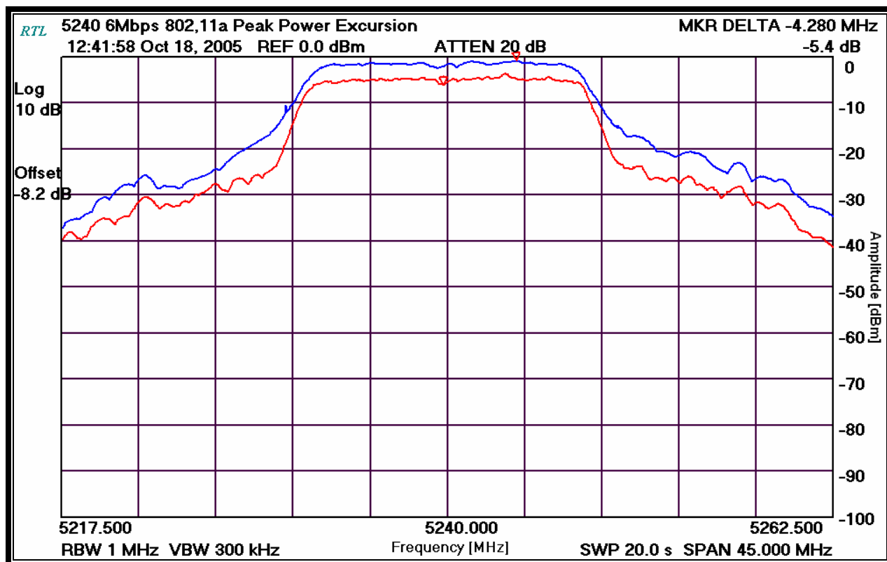
Plot 15-3: Peak Power Excursion: Channel 48 (5240 MHz – 6 Mb/s)
