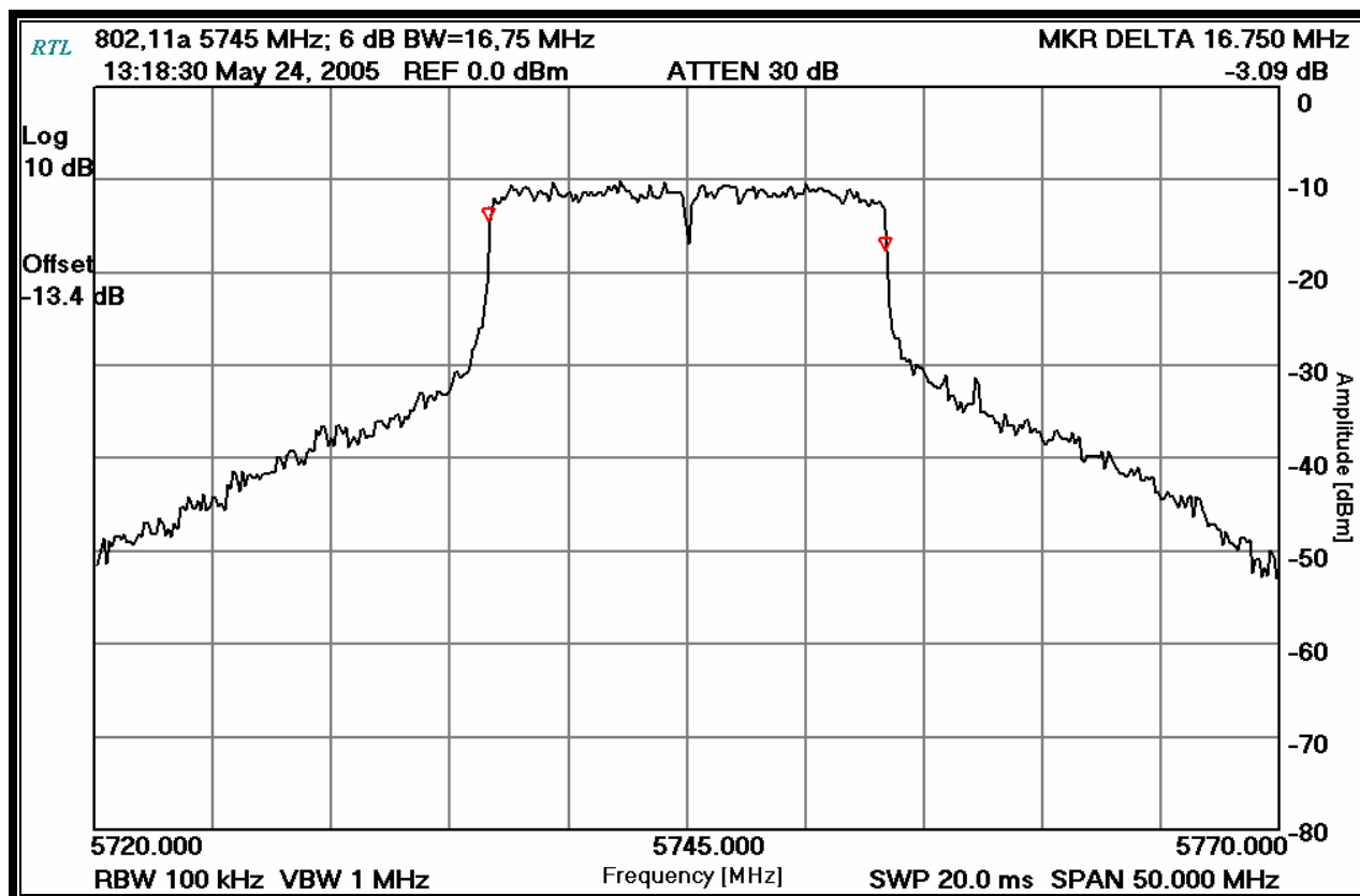
Plot 20-1: 6 dB Bandwidth (TX Frequency: 5745 MHz – 6 Mbs)
