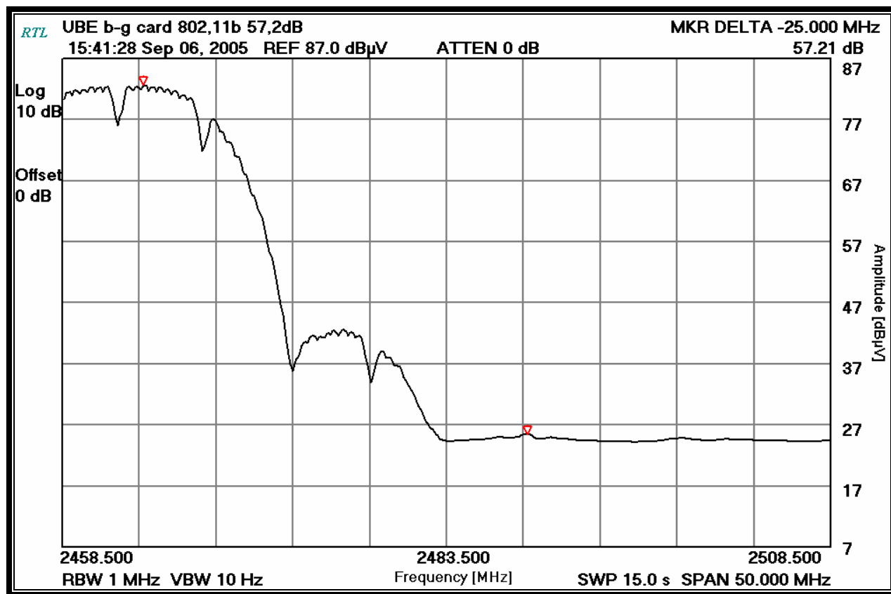
Plot 4-2: Upper Band Edge: Average Measurement Channel 11 (TX Frequency: 2462 MHz – 1 Mbps) Omni Antenna
