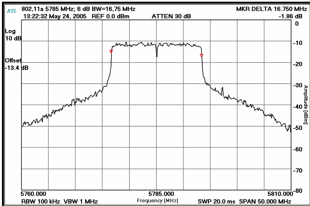
Plot 20-2: 6 dB Bandwidth (TX Frequency: 5785 MHz – 6 Mbs)
