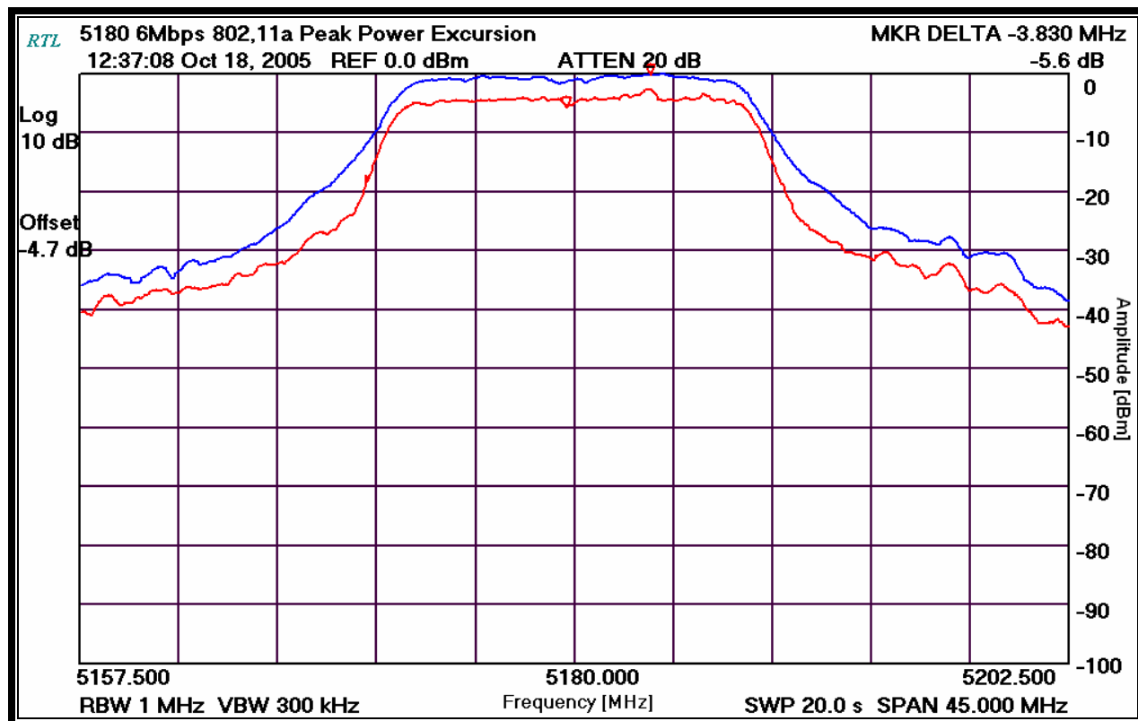
Plot 15-1: Peak Power Excursion: Channel 36 (5180 MHz – 6 Mb/s)
