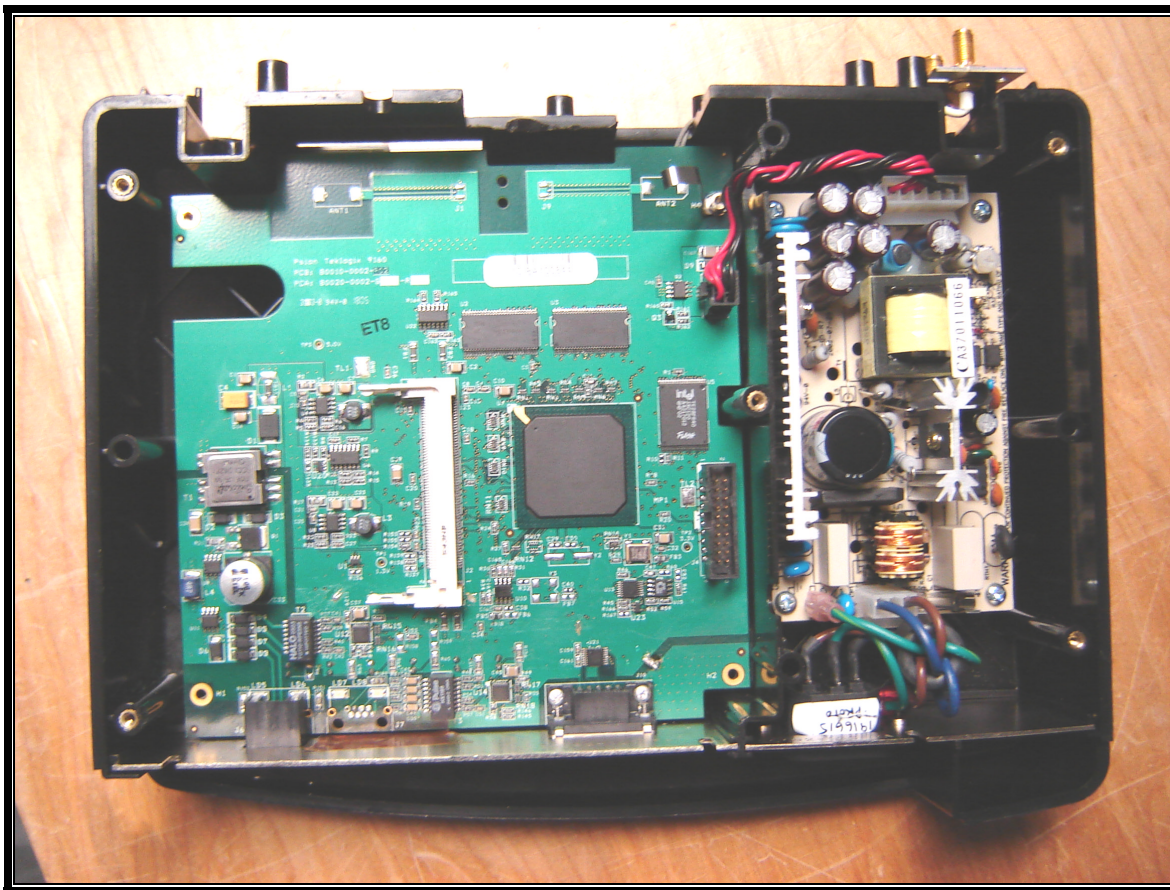
Photograph 18: Inside Bottom View with PCB's
