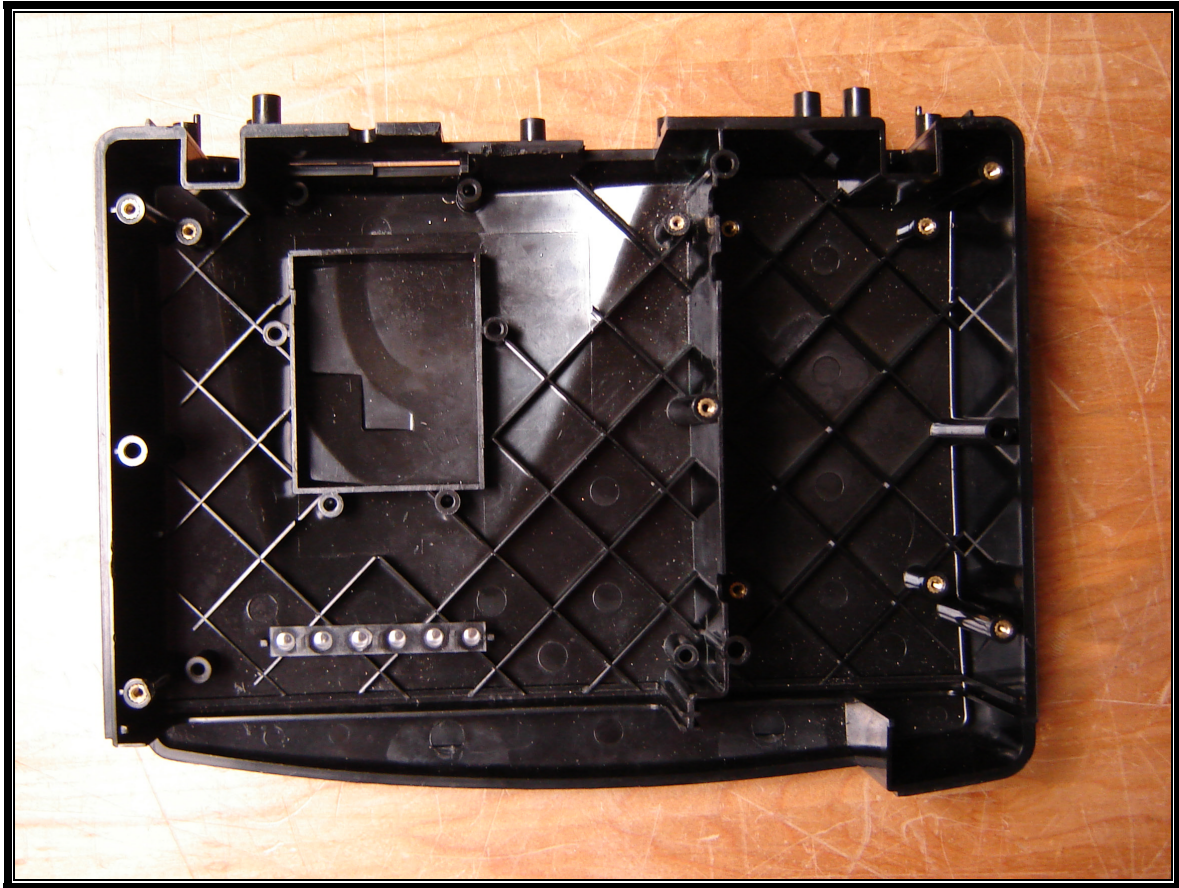
Photograph 19: Inside Bottom View PCB's Removed
