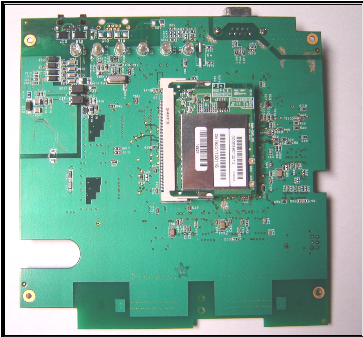
Photograph 20: Main PCB; Top View – with Radio Card
