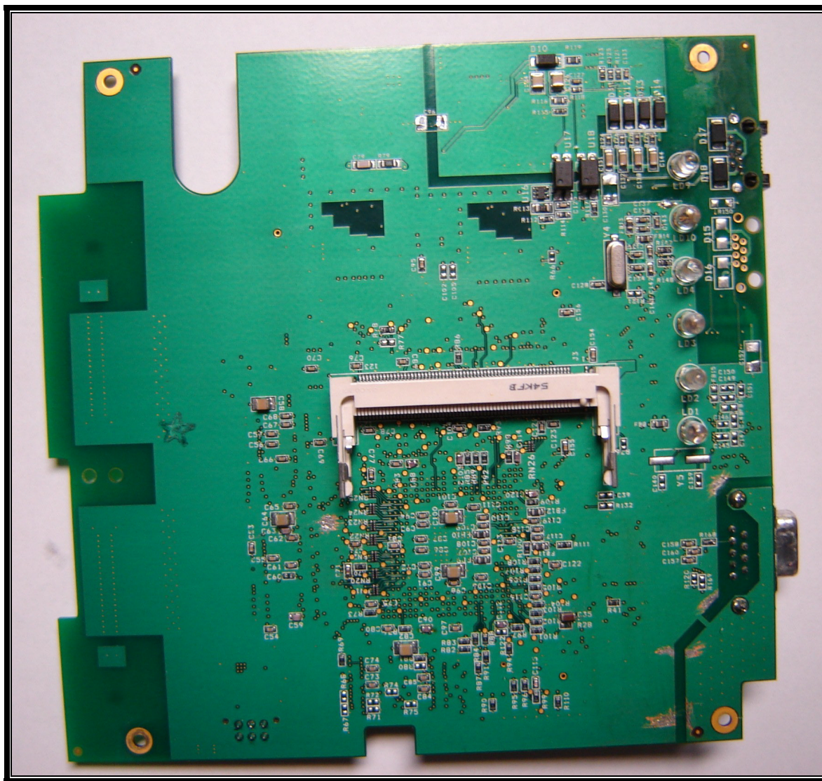
Photograph 21: Main PCB; Top View – Radio Removed
