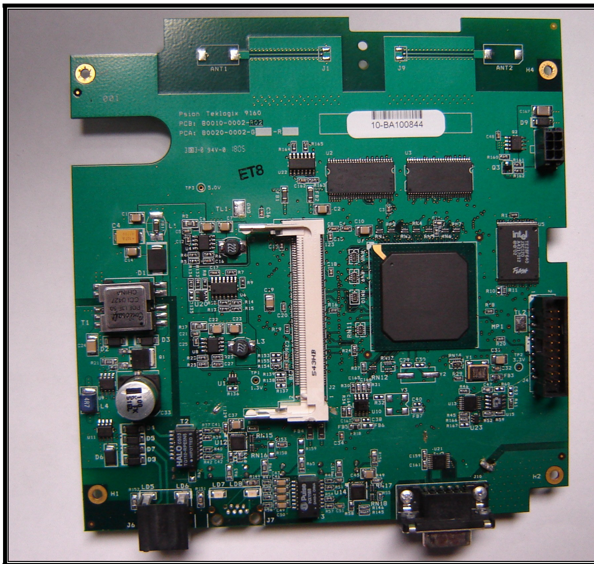
Photograph 22: Main PCB Bottom View
