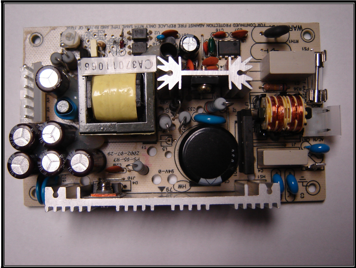
Photograph 24: Bottom of Power Supply PCB
