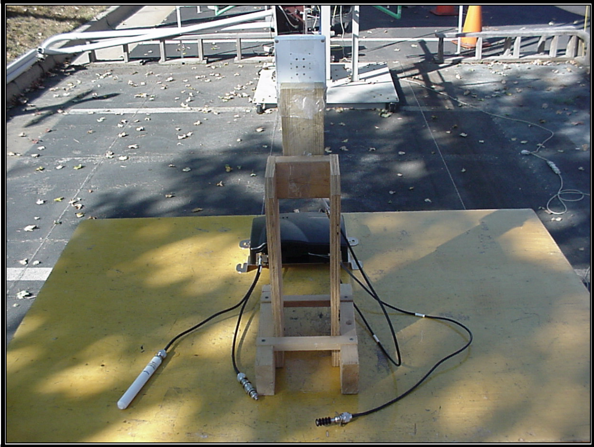
Photograph 2: Radiated Testing – 8.5 dBi Patch Rear View
