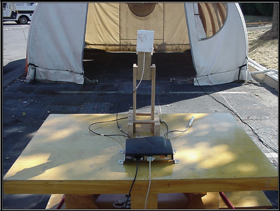
Photograph 1: Radiated Testing – 8.5 dBi Patch Front View
