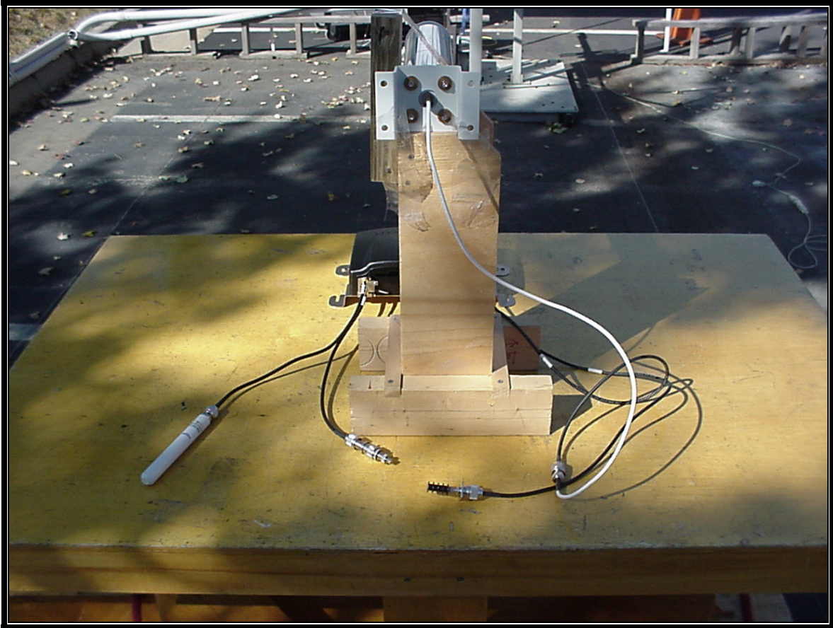
Photograph 6: Radiated Testing – 14 dBi YAGI Rear View
