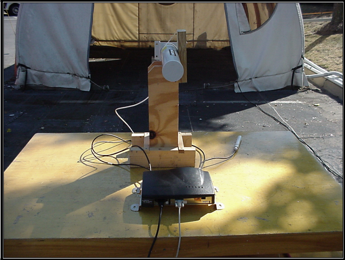
Photograph 5: Radiated Testing – 14 dBi YAGI Front View
