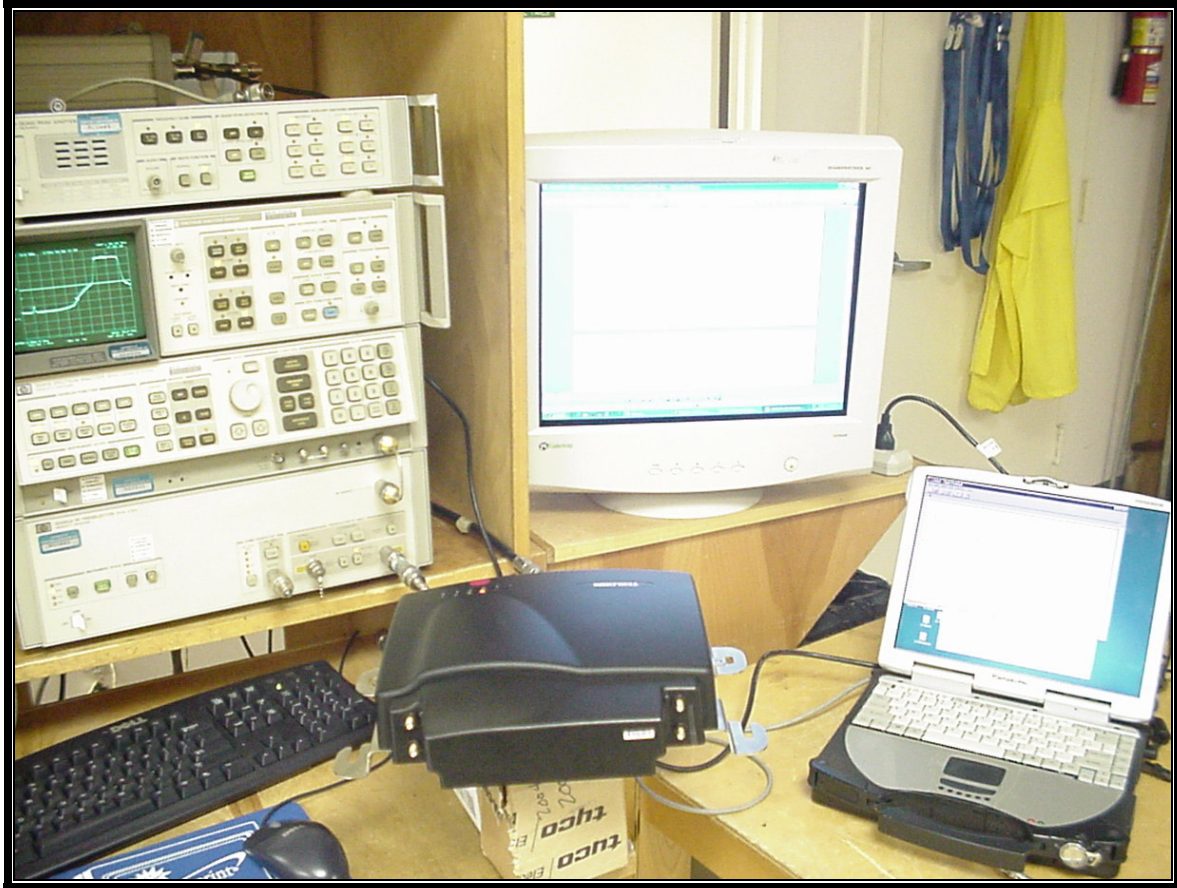
Photograph 11: Conducted Antenna Port Testing
