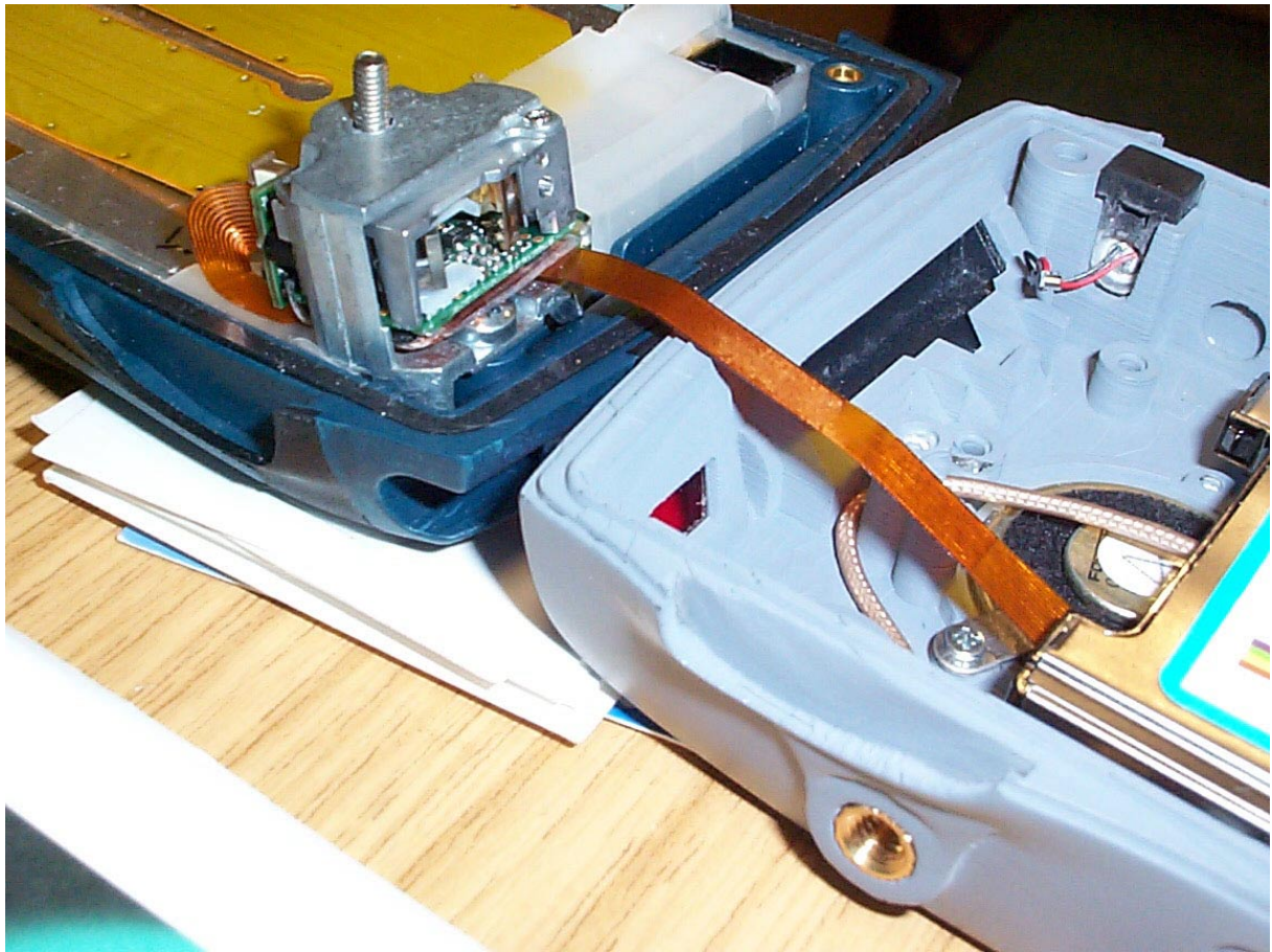
Scanner Assembly
