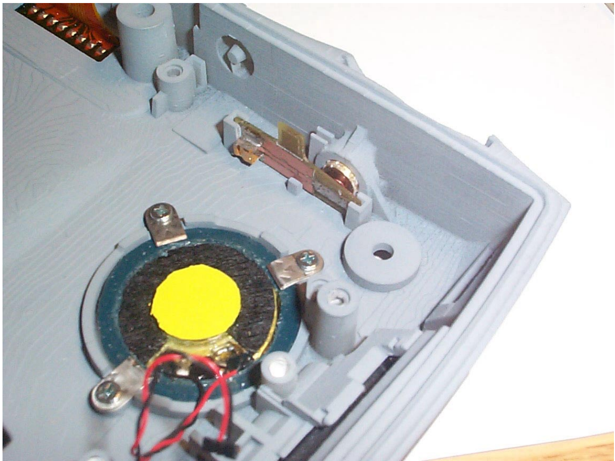
External Antenna PCB and Insert
