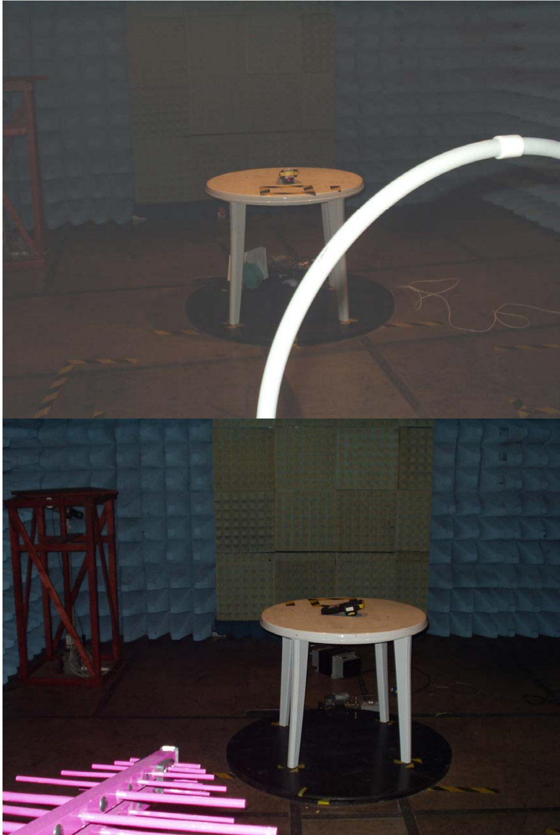
Photograph of the EUT (handheld) as viewed from in front of the loop / bilog antennas, site M.
