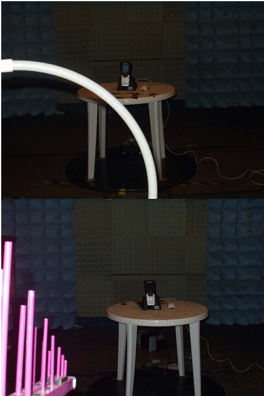
Photograph of the EUT (docked) as viewed from in front of the loop / bilog antennas, site M.
