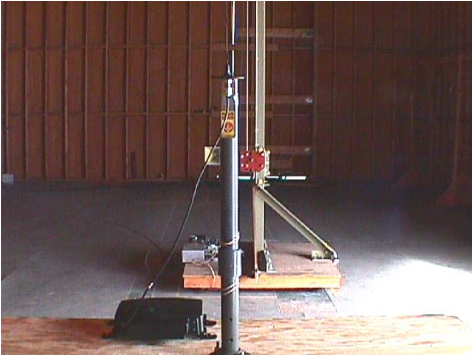
Test Configuration #4: Psion Teklogix Model No.: 9150-RA2020 + Larsen Antenna, Model FB45T2400, Gain: 7.2 dBi
