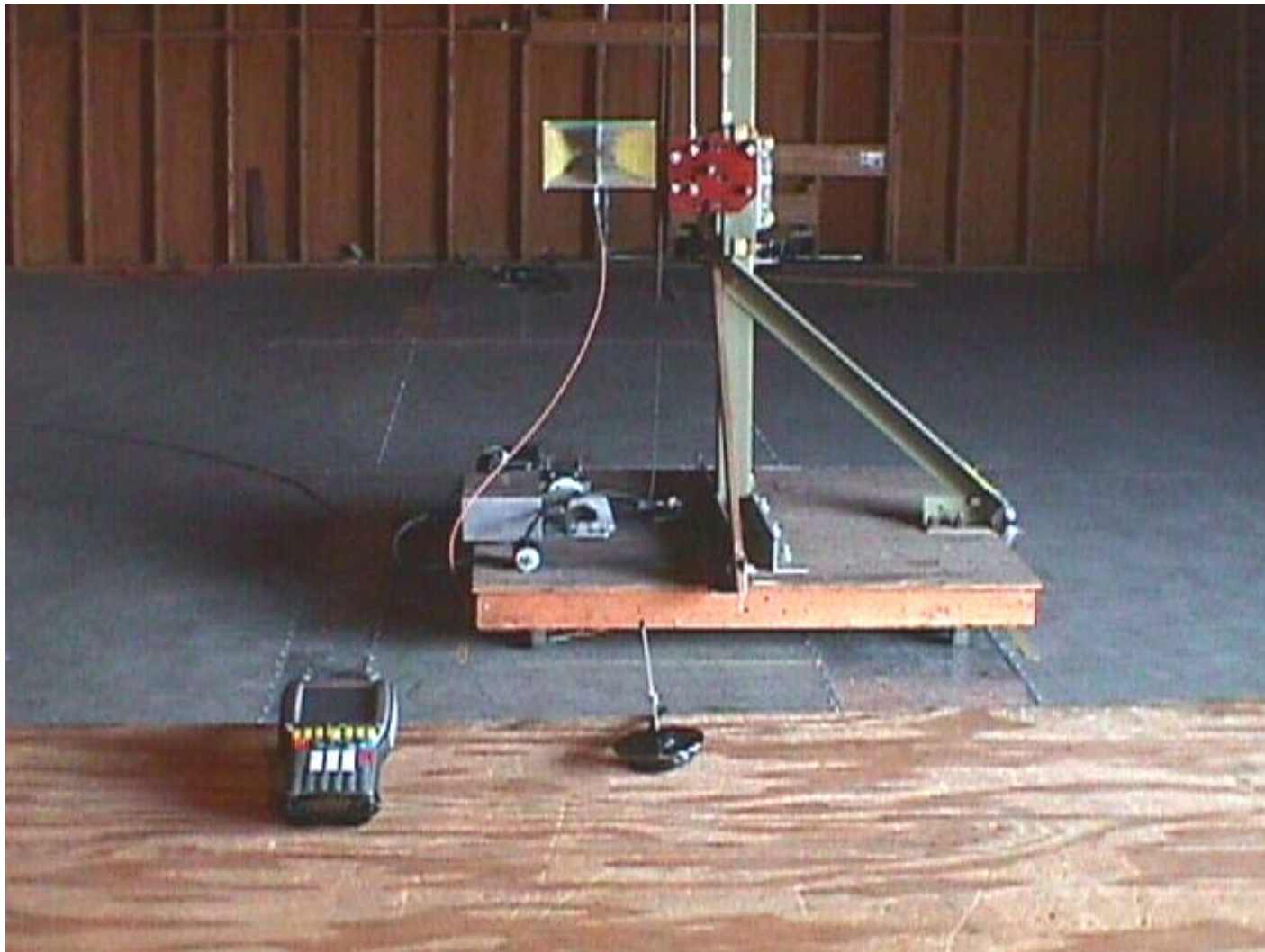
Test Configuration #2: Psion Teklogix Model RA2020 + Mobile Mark Antenna, Model IMAG5-2400, Gain: 5 dBi
