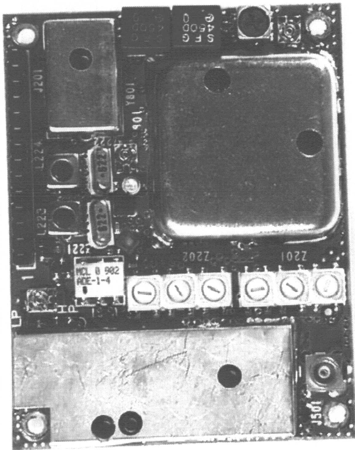
TRX 7370 RADIO
