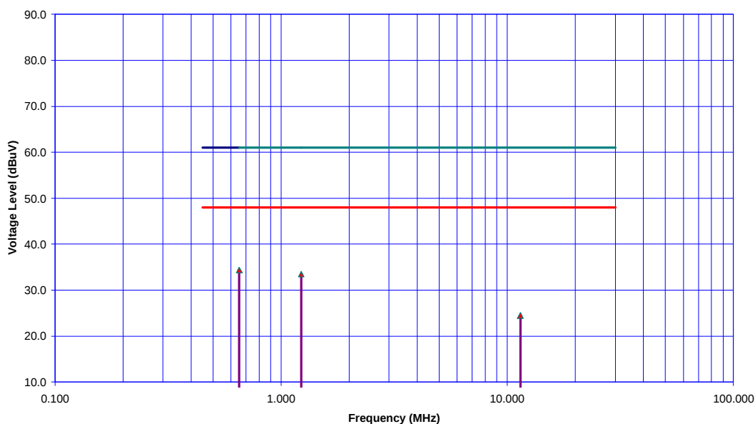
AC Conducted Emissions - Line #2 (Neutral) Teklogix TRX7431 with 8260 Vehicle Terminal
