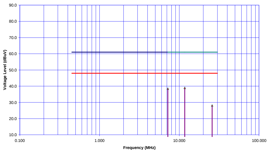
AC Conducted Emissions - Line #2 (Neutral) Teklogix TRX7431 with 9150 Base Station
