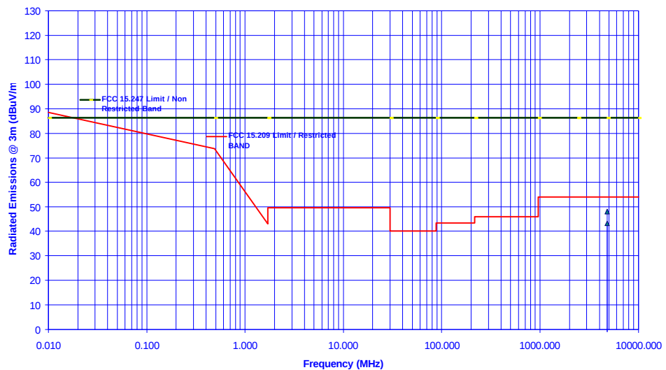
Teklogix TRX7431 with Test Jig Transmitter Radiated Emissions Measurements at 3 Meter OFTS TRANSMIT Freq.: 2412 MHz
