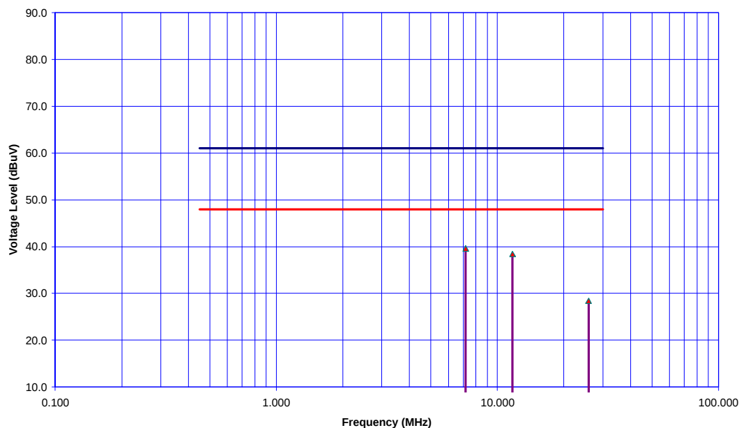
AC Conducted Emissions - Line #1 (Hot) Teklogix TRX7431 with 9150 Base Station
