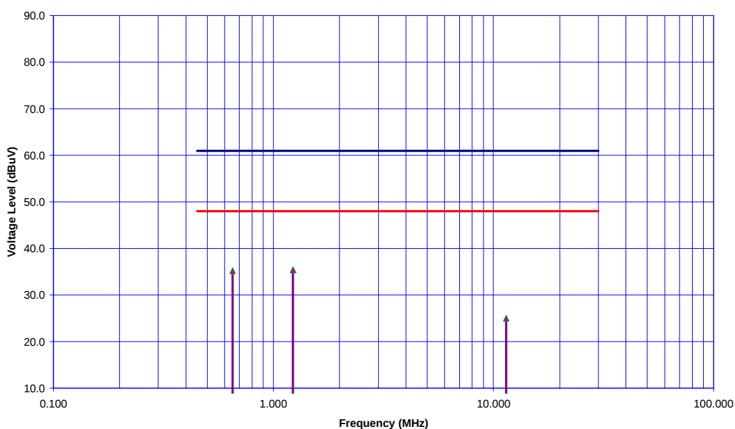
AC Conducted Emissions - Line #2 (Neutral) Teklogix TRX7431 with 8260 Vehicle Terminal
