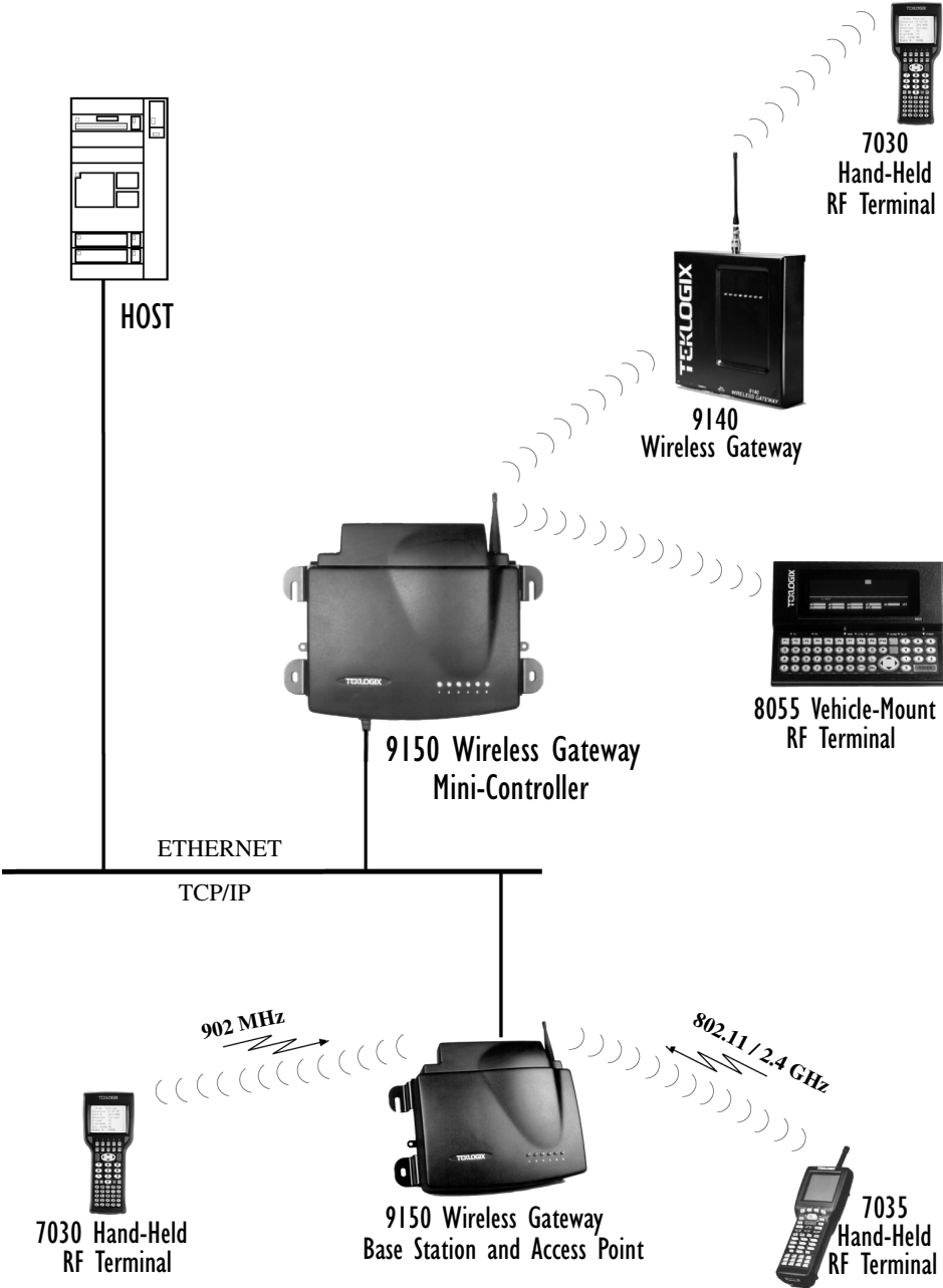
Figure 5.1 9150 Mini-Controller Configuration
