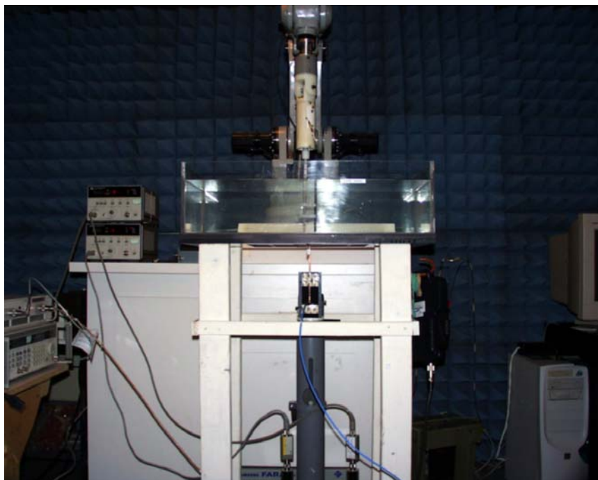
< Thermal transfer calibration and system verification setup >
