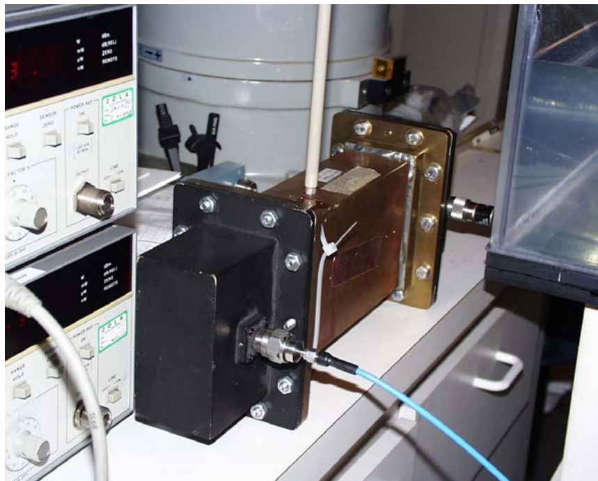
< Free space calibration setup >
