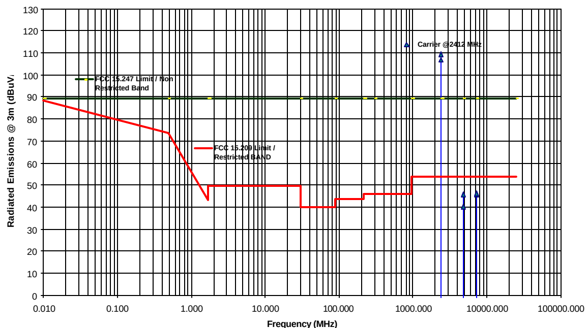
Transmitter Radiated Emissions Measurements at 3 Meter OETS NETPAD + TRX7431 (DSSS Modular Transceiver), Model NETPAD RLAN TRANSMIT Freq.: 2412 MHz, Modulation CCK @ 11 Mbps
