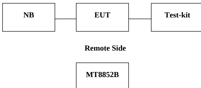
Fig. 2-1 Radiated Emission
