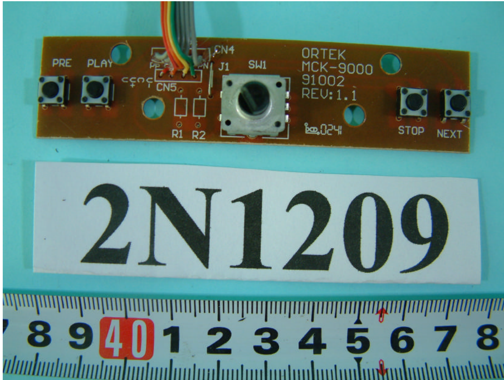
Front side of Media Control Board
