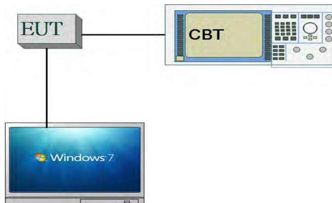
Fig. 2-2 Conducted (Antenna Port) Configuration
