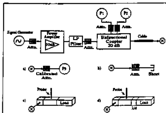
Fig. 2. Setup for calibration in waveguides (air). Measurements c and d to calibrate the power meters P_1 and P_2 . P_3 is a high-precision meter. Probe measurements c and d with different distances to load.
