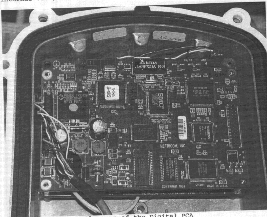
Close-up of the Digital PCA
