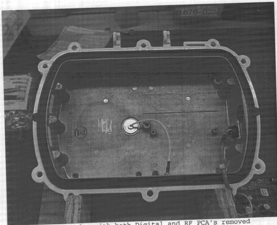
Close-Up of the RF PCA removed from the housing
