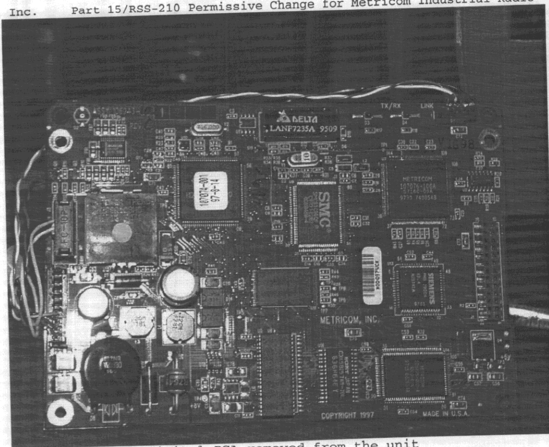
Digital PCA removed from the unit
