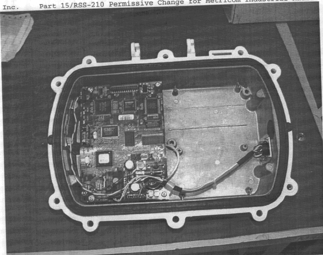
Internal view, showing Digital PCA & Other half of housing removed
