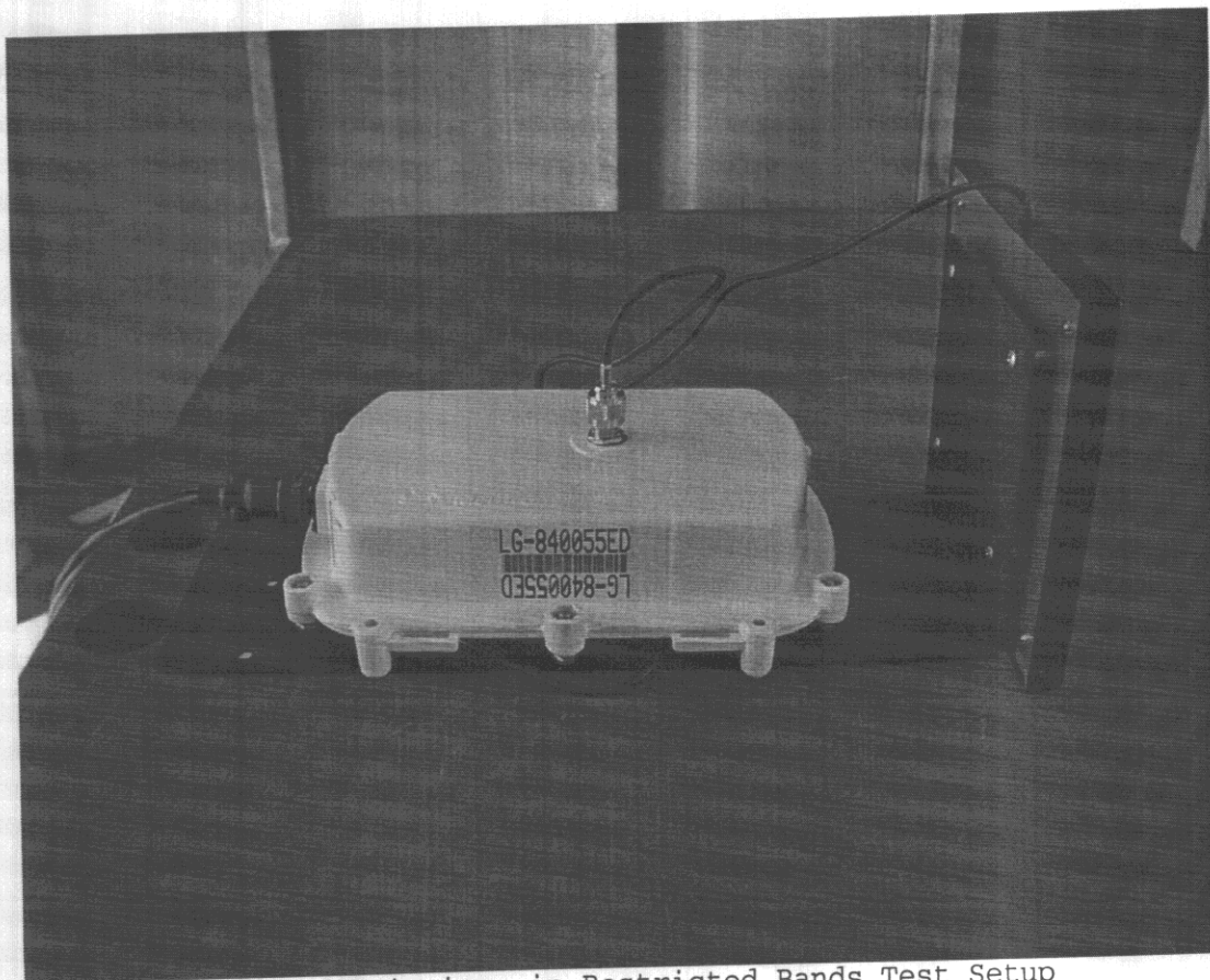
Radiated Emissions in Restricted Bands Test Setup
