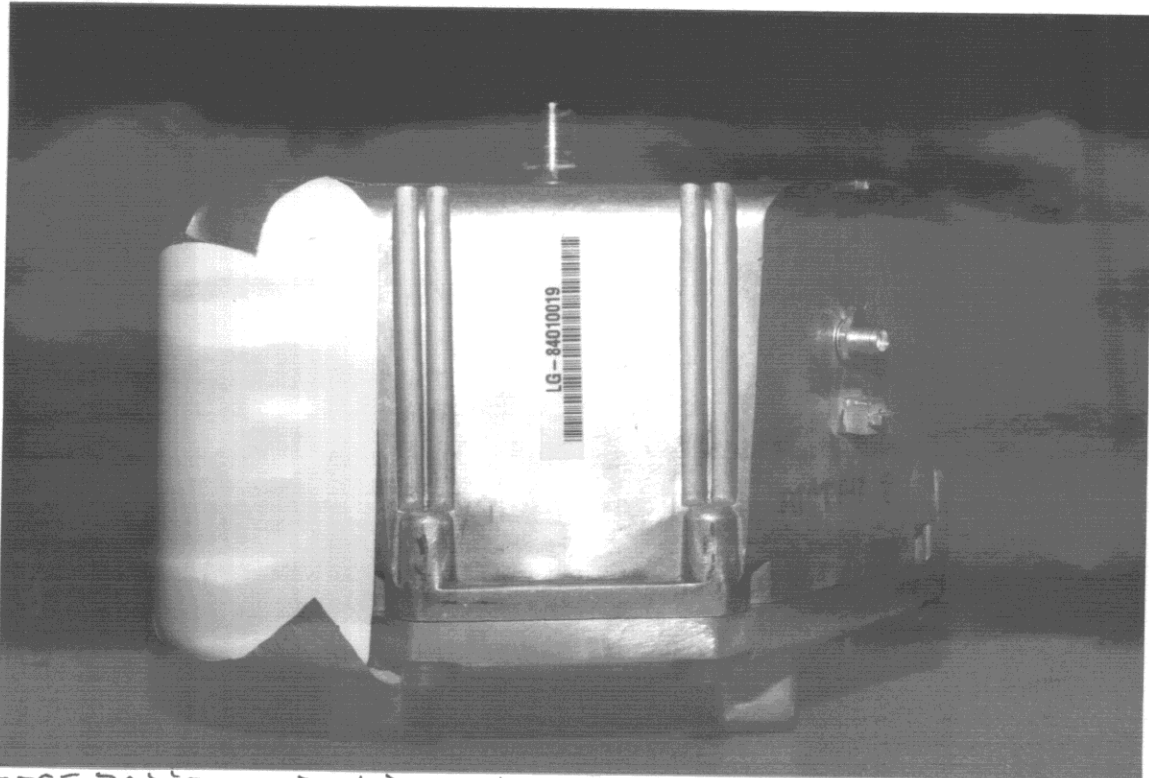
TEST RADIO, END VIEW SHOWING MODIFICATION FOR 2.4 GHZ CONDUCTED TESTS
