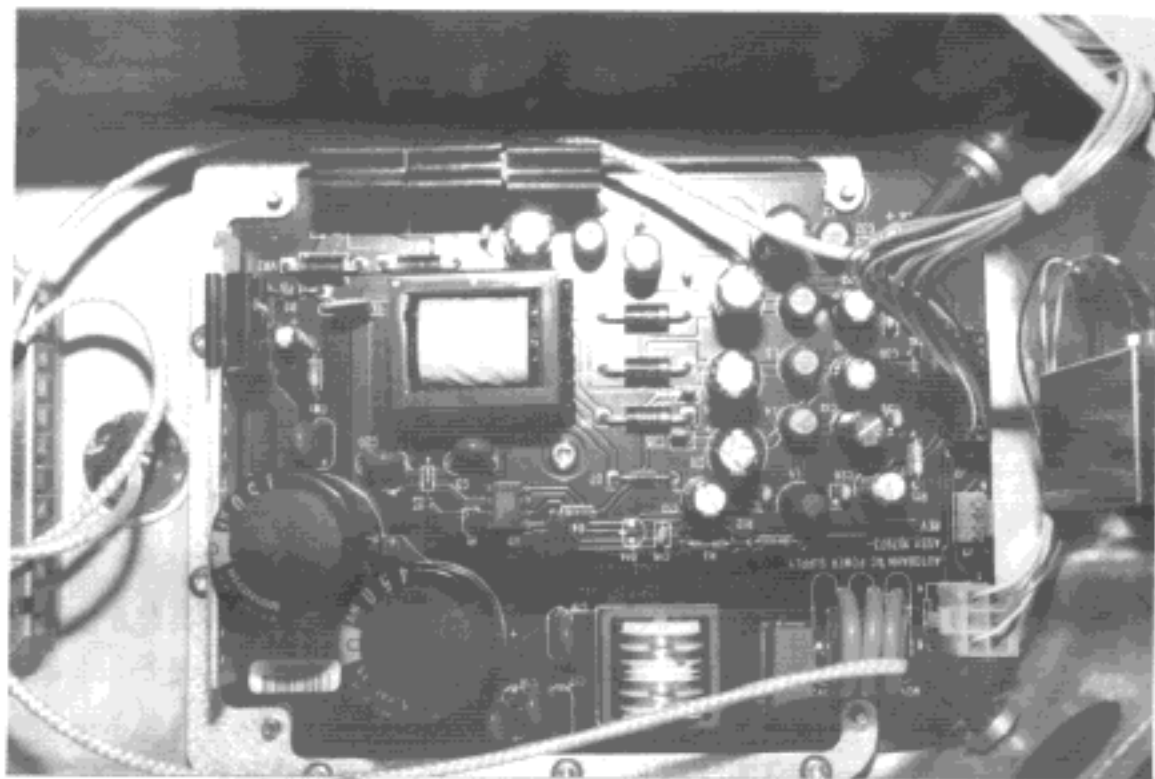
CLOSE UP, POWER SUPPLY
