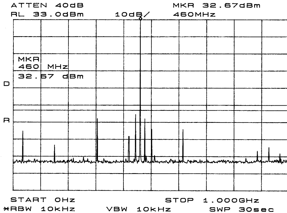
Figure 2: Emissions at Antenna Terminal
