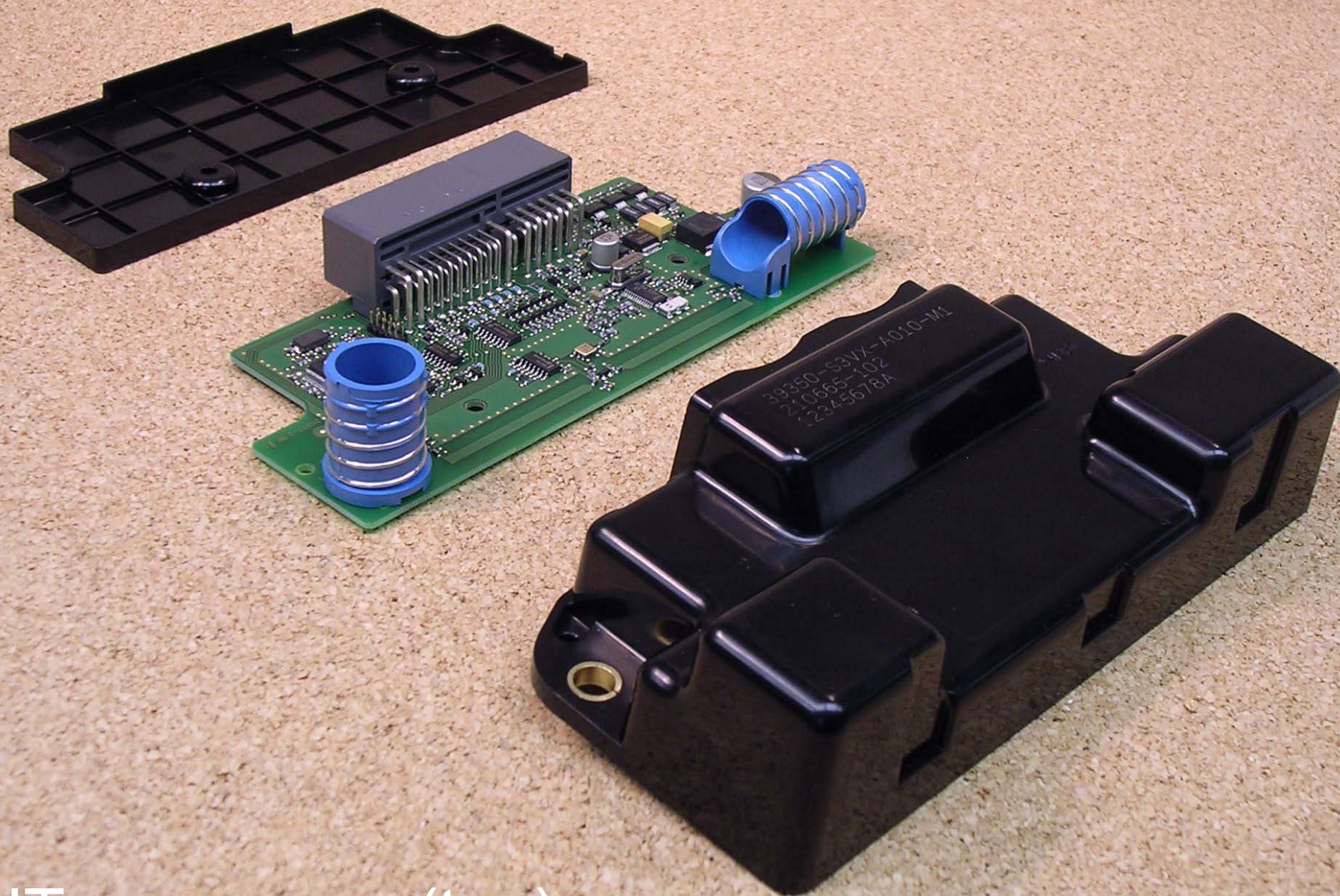
DUT case open (top)
