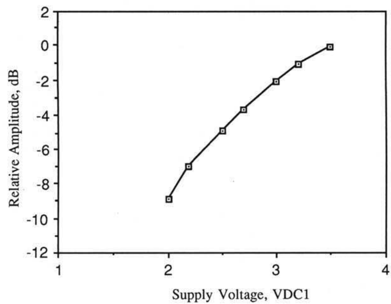
Figure 6.4. Relative emission at 315.0 MHz vs. supply voltage. (CW emission)
