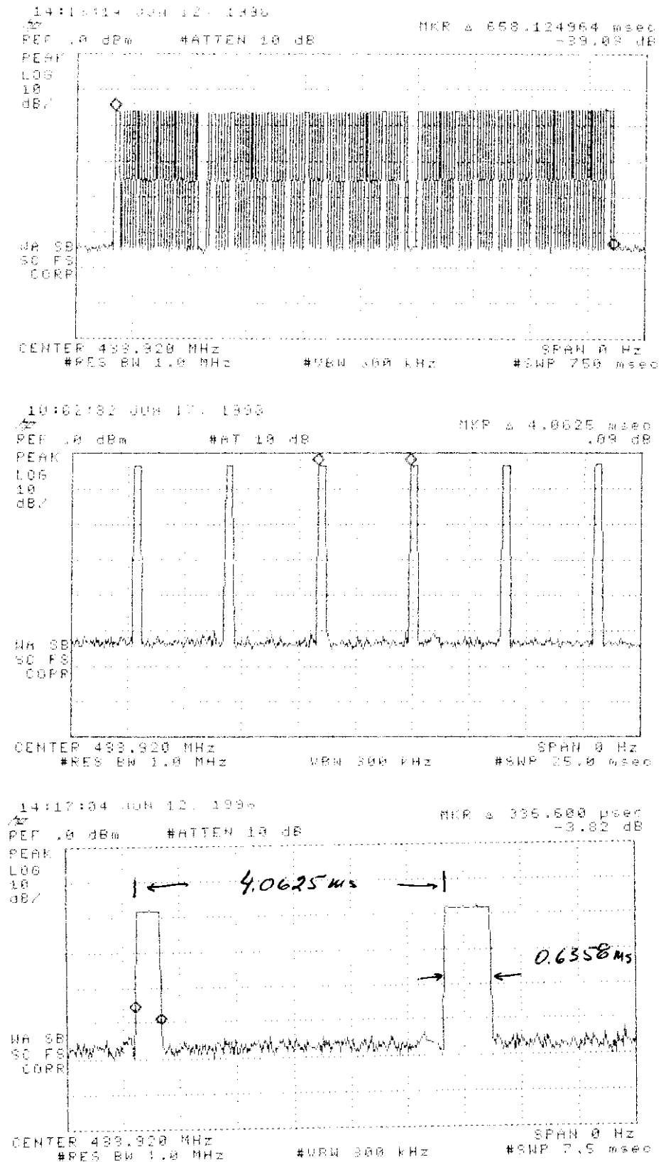
Figure 6.1. Transmissions modulation characteristics: (top) complete transmission, (center) expanded word, (bottom) expanded bits.
