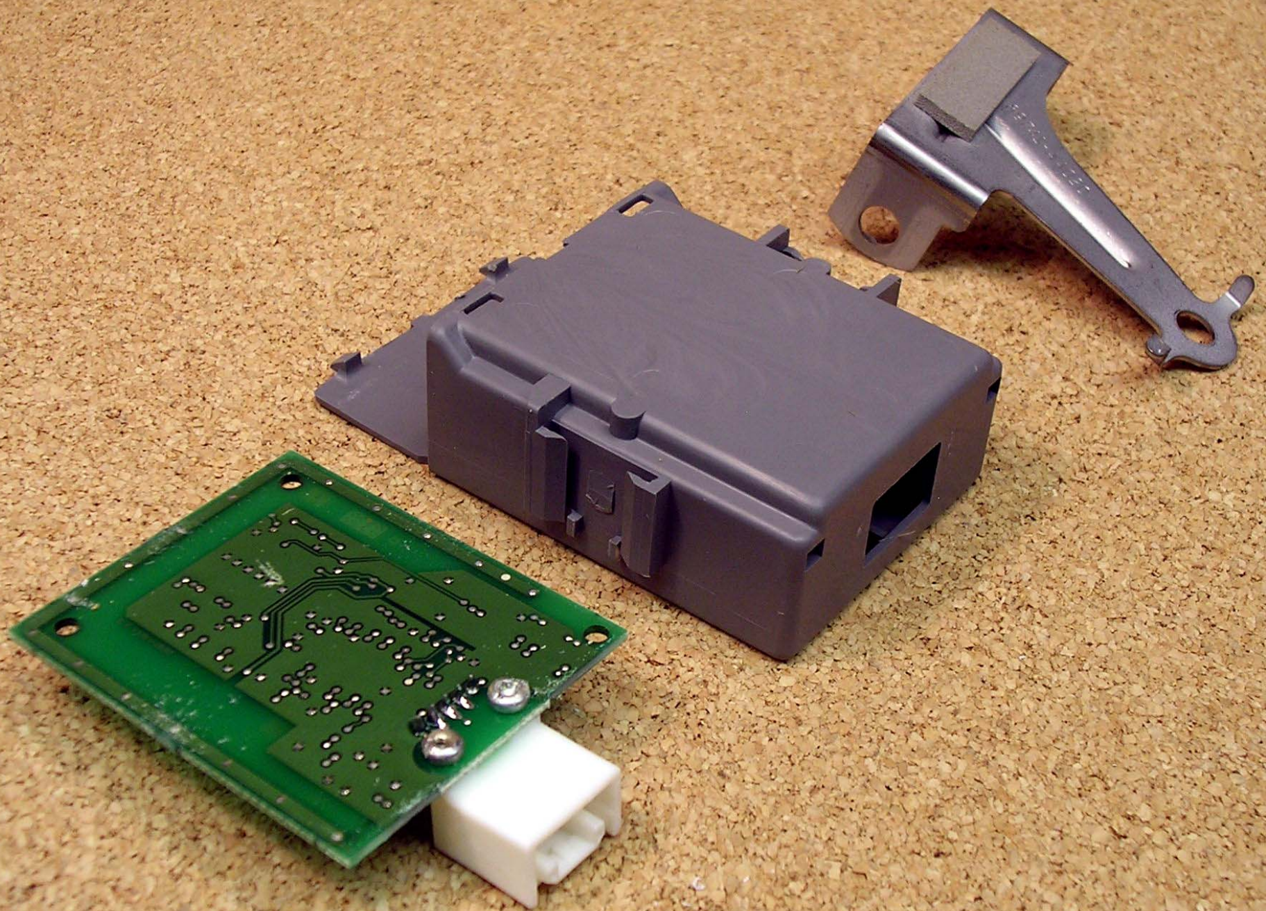
DUT case open (bottom)
