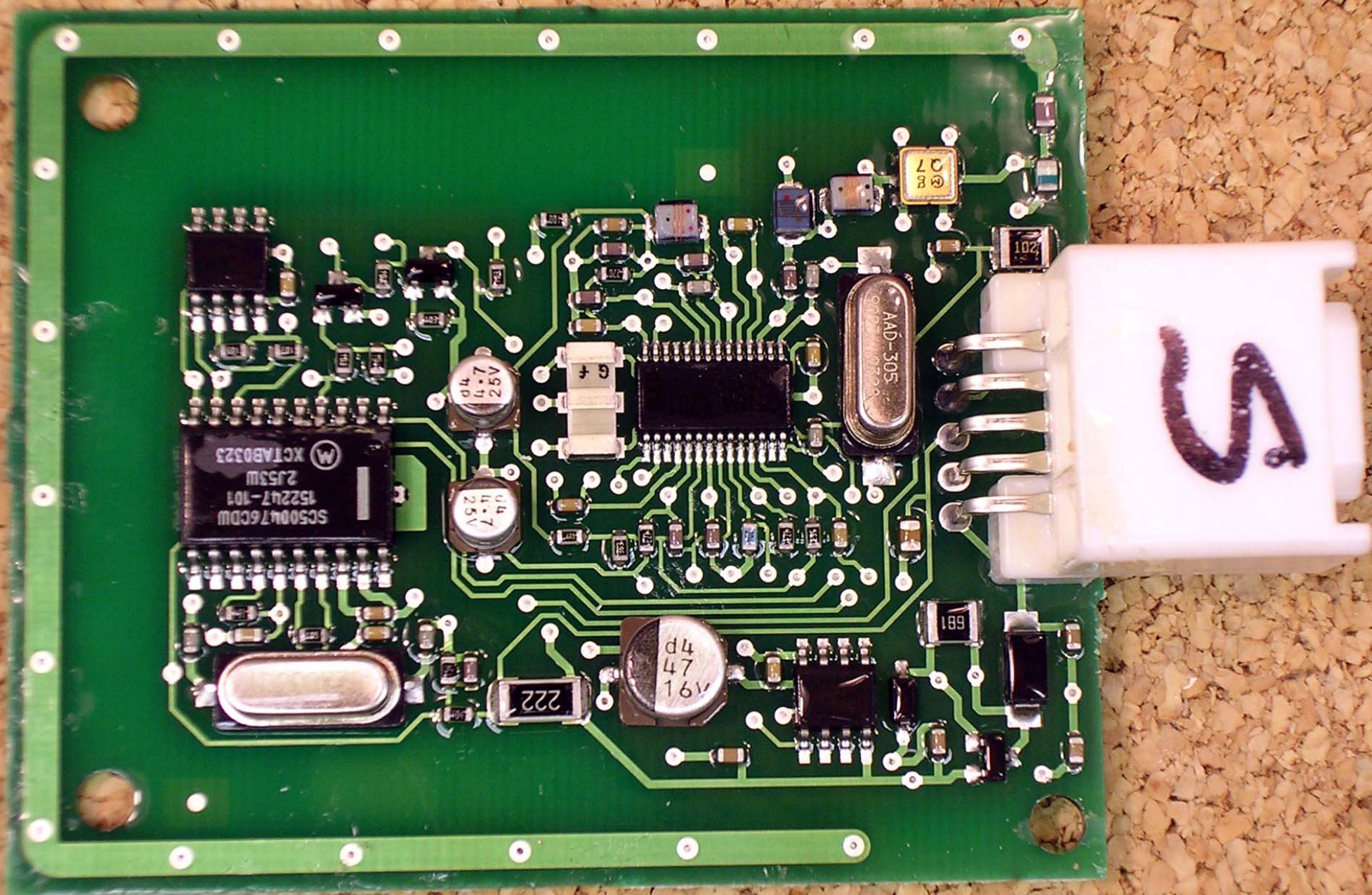
PCB (top)
